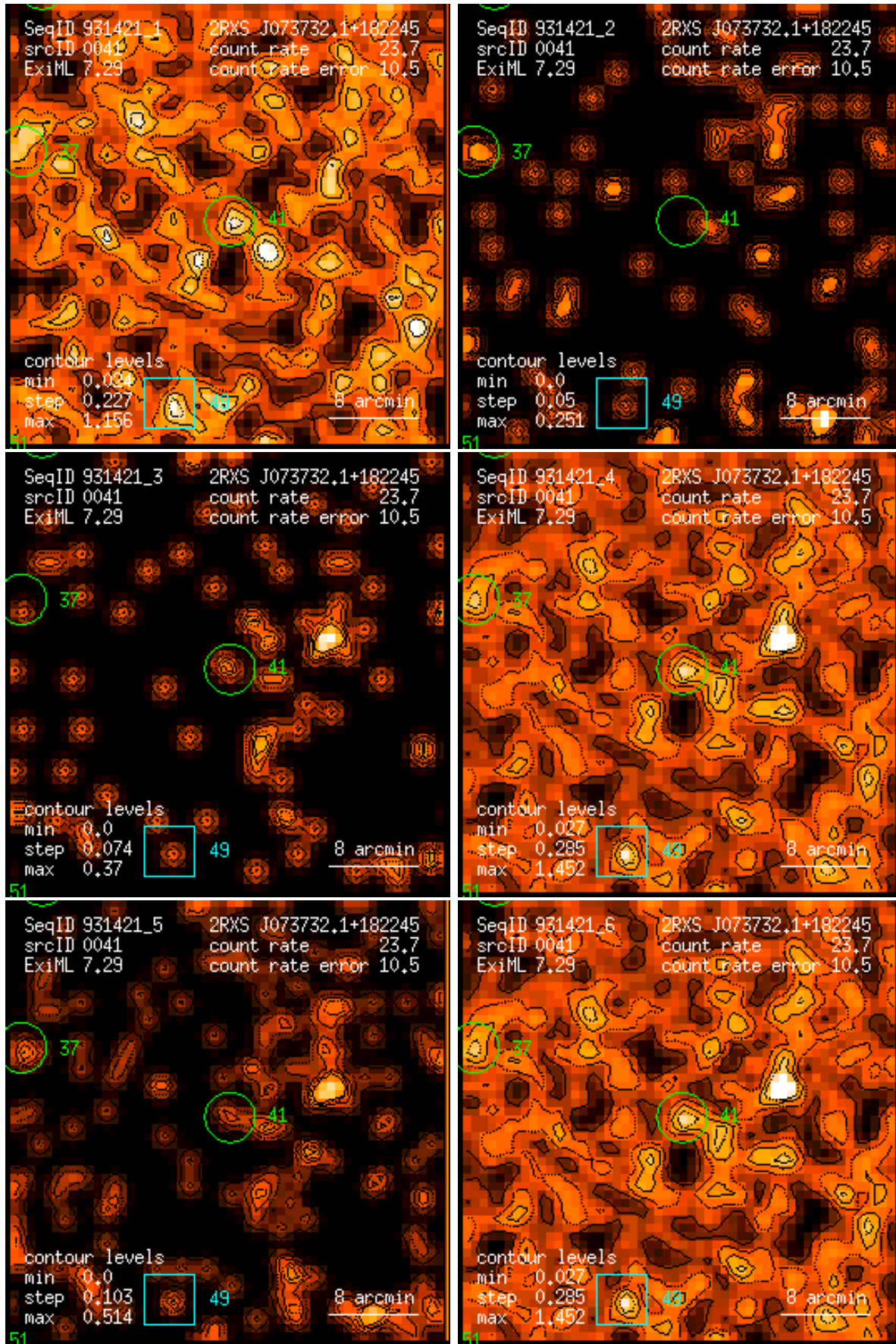
Figure 41: RASS 931421: detection 0041: band rate images, Gaussian filter: (1) PSPC channels 11 – 41, (2) 52 – 90, (3) 91 – 201, (4) 11 – 235, (5) 52 – 201, (6) 11 – 201. Broad band rates in counts/ks. Band rate contour levels in counts/ks/arcmin 2 .
