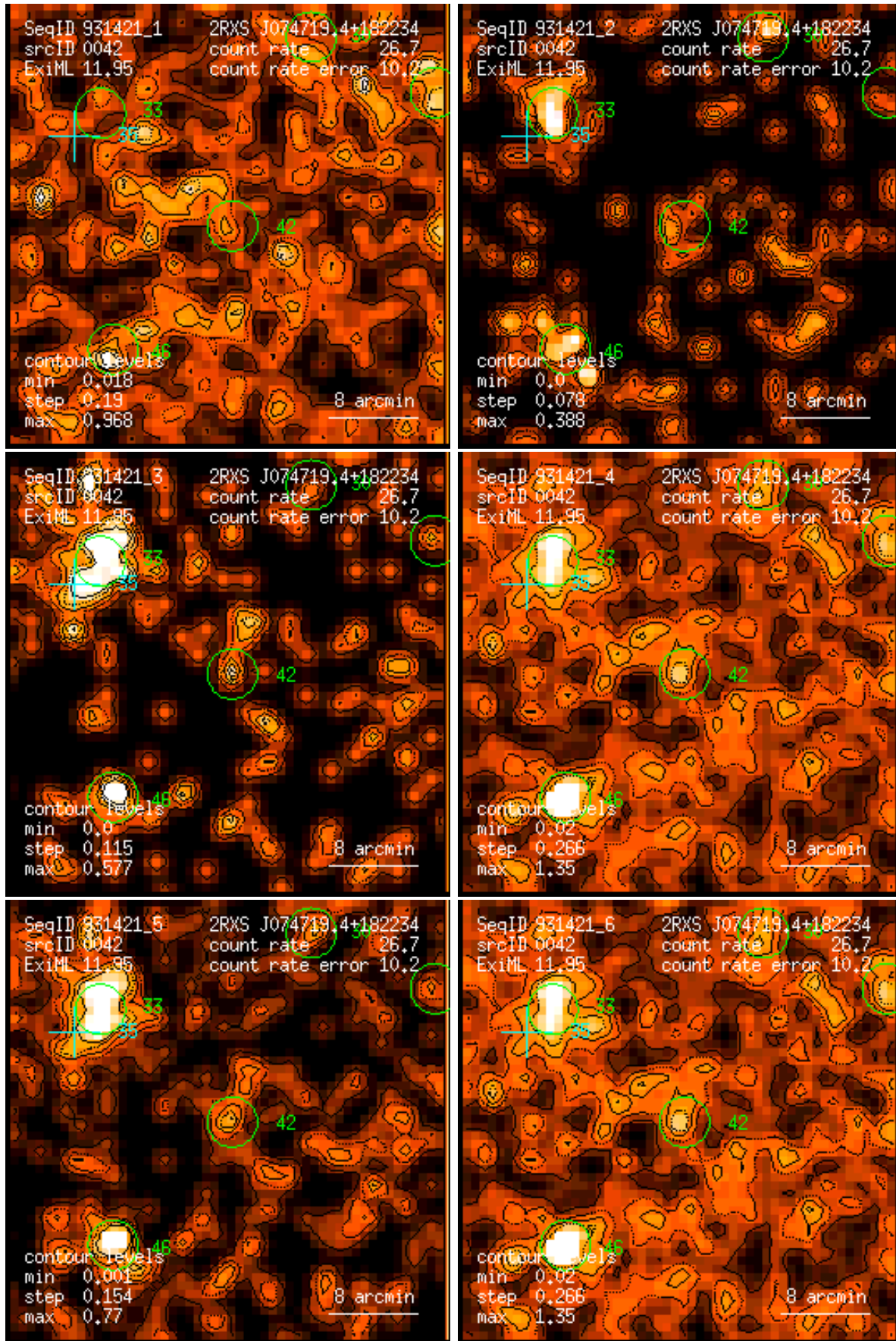
Figure 42: RASS 931421: detection 0042: band rate images, Gaussian filter: (1) PSPC channels 11 – 41, (2) 52 – 90, (3) 91 – 201, (4) 11 – 235, (5) 52 – 201, (6) 11 – 201. Broad band rates in counts/ks. Band rate contour levels in counts/ks/arcmin 2 .
