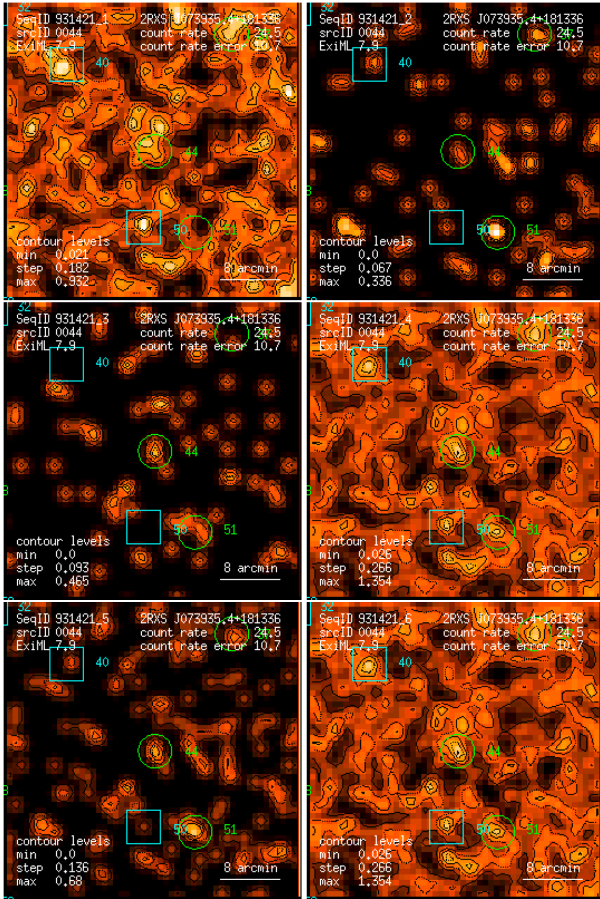
Figure 44: RASS 931421: detection 0044: band rate images, Gaussian filter: (1) PSPC channels 11 – 41, (2) 52 – 90, (3) 91 – 201, (4) 11 – 235, (5) 52 – 201, (6) 11 – 201. Broad band rates in counts/ks. Band rate contour levels in counts/ks/arcmin 2 .
