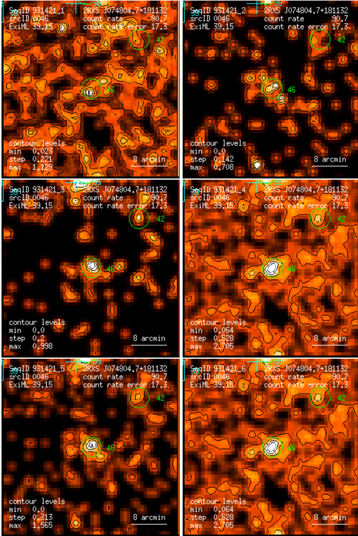
Figure 46: RASS 931421: detection 0046: band rate images, Gaussian filter: (1) PSPC channels 11 – 41, (2) 52 – 90, (3) 91 – 201, (4) 11 – 235, (5) 52 – 201, (6) 11 – 201. Broad band rates in counts/ks. Band rate contour levels in counts/ks/arcmin 2 .
