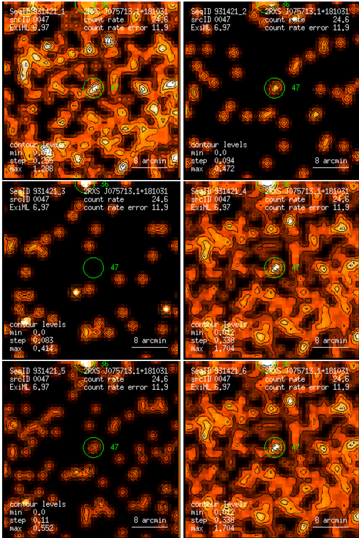
Figure 47: RASS 931421: detection 0047: band rate images, Gaussian filter: (1) PSPC channels 11 – 41, (2) 52 – 90, (3) 91 – 201, (4) 11 – 235, (5) 52 – 201, (6) 11 – 201. Broad band rates in counts/ks. Band rate contour levels in counts/ks/arcmin 2 .
