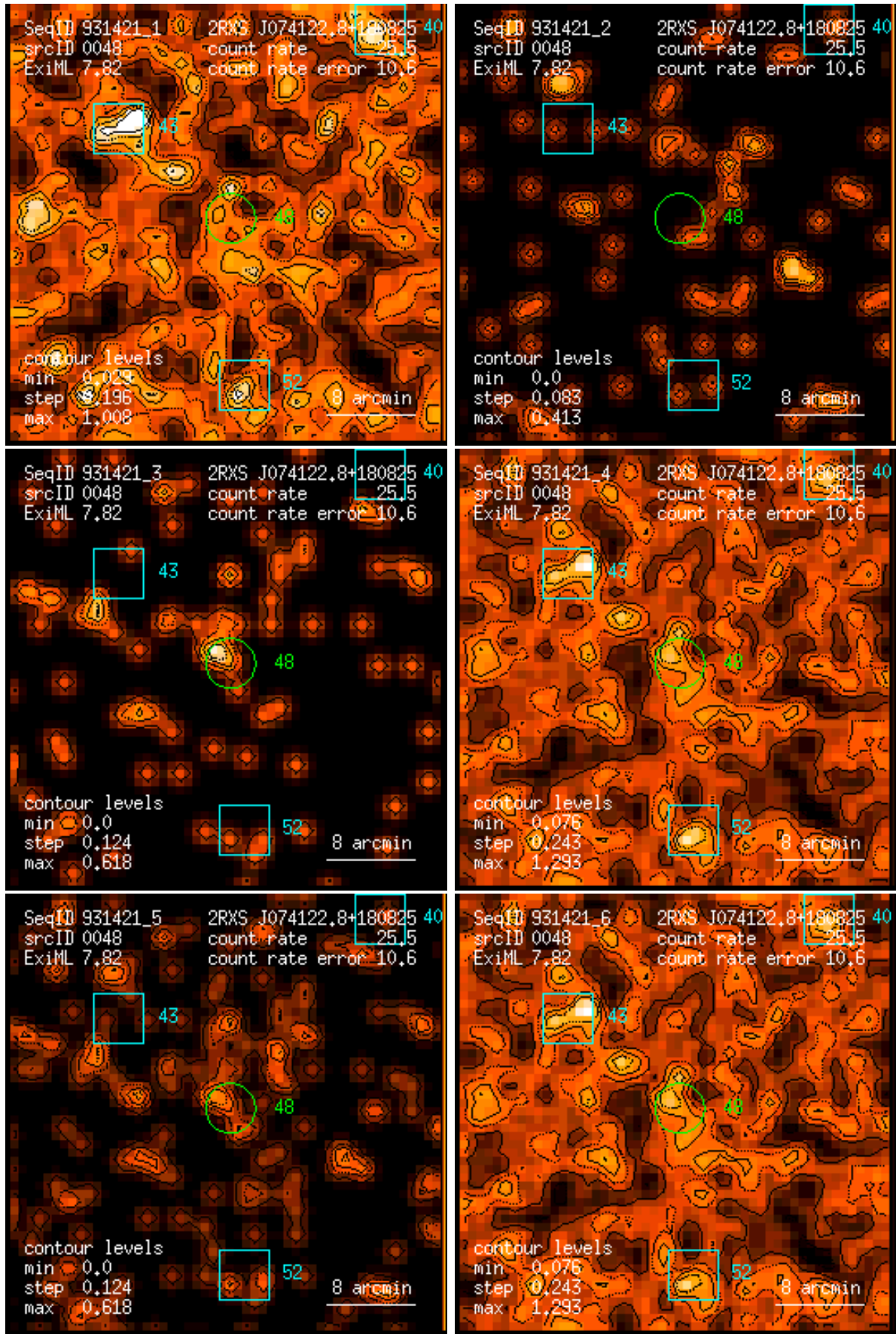
Figure 48: RASS 931421: detection 0048: band rate images, Gaussian filter: (1) PSPC channels 11 – 41, (2) 52 – 90, (3) 91 – 201, (4) 11 – 235, (5) 52 – 201, (6) 11 – 201. Broad band rates in counts/ks. Band rate contour levels in counts/ks/arcmin 2 .
