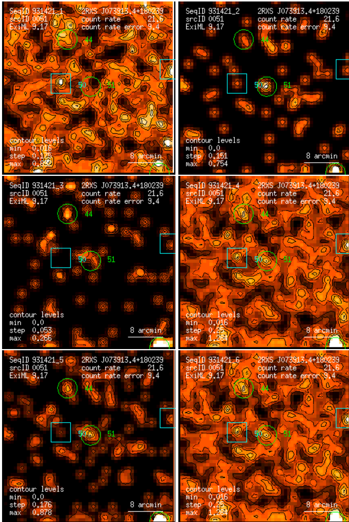
Figure 51: RASS 931421: detection 0051: band rate images, Gaussian filter: (1) PSPC channels 11 – 41, (2) 52 – 90, (3) 91 – 201, (4) 11 – 235, (5) 52 – 201, (6) 11 – 201. Broad band rates in counts/ks. Band rate contour levels in counts/ks/arcmin 2 .
