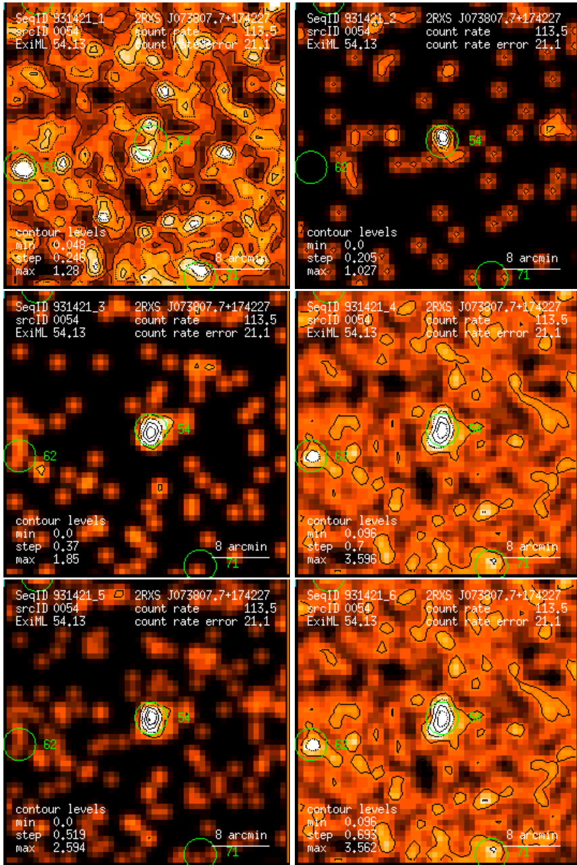
Figure 54: RASS 931421: detection 0054: band rate images, Gaussian filter: (1) PSPC channels 11 – 41, (2) 52 – 90, (3) 91 – 201, (4) 11 – 235, (5) 52 – 201, (6) 11 – 201. Broad band rates in counts/ks. Band rate contour levels in counts/ks/arcmin 2 .
