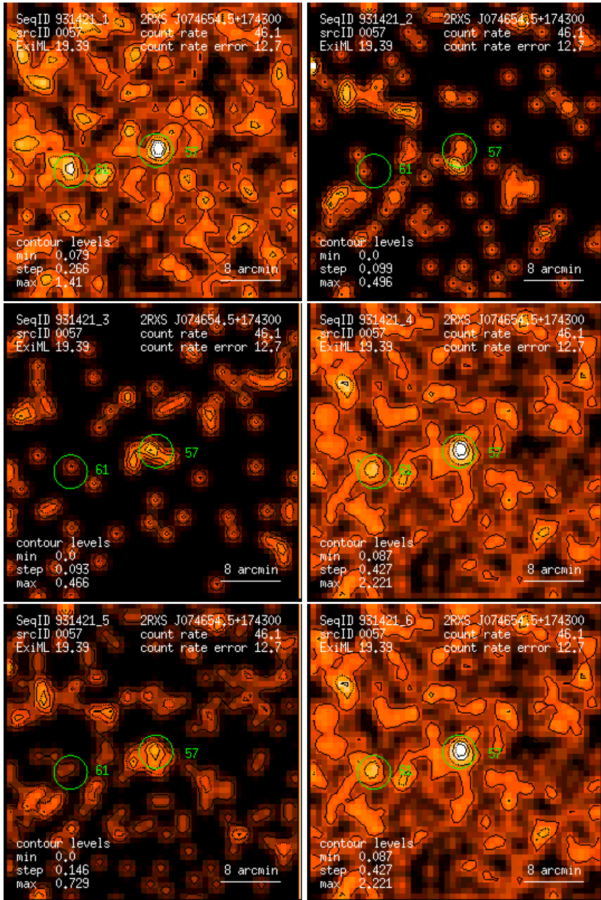
Figure 57: RASS 931421: detection 0057: band rate images, Gaussian filter: (1) PSPC channels 11 – 41, (2) 52 – 90, (3) 91 – 201, (4) 11 – 235, (5) 52 – 201, (6) 11 – 201. Broad band rates in counts/ks. Band rate contour levels in counts/ks/arcmin 2 .
