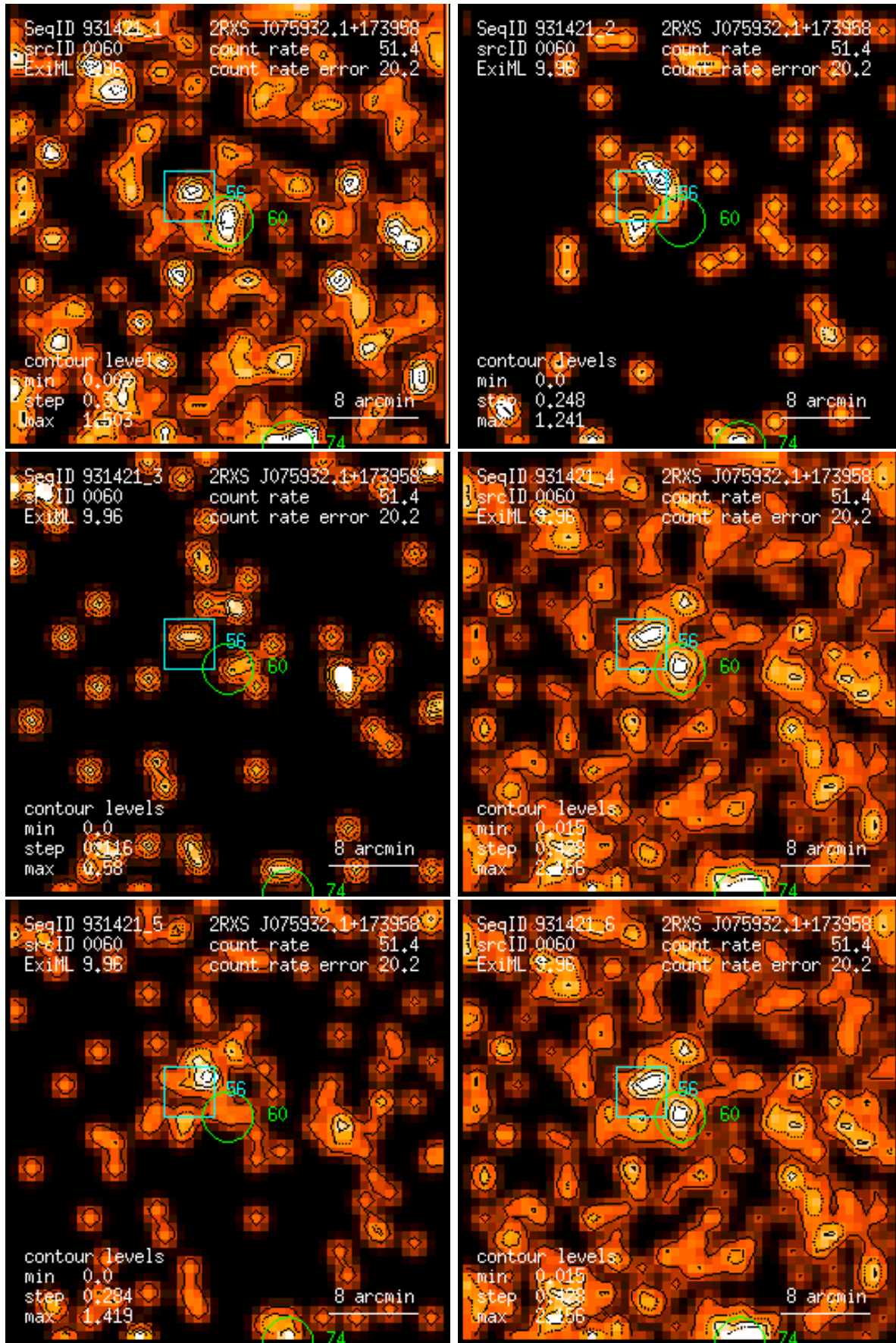
Figure 60: RASS 931421: detection 0060: band rate images, Gaussian filter: (1) PSPC channels 11 – 41, (2) 52 – 90, (3) 91 – 201, (4) 11 – 235, (5) 52 – 201, (6) 11 – 201. Broad band rates in counts/ks. Band rate contour levels in counts/ks/arcmin 2 .
