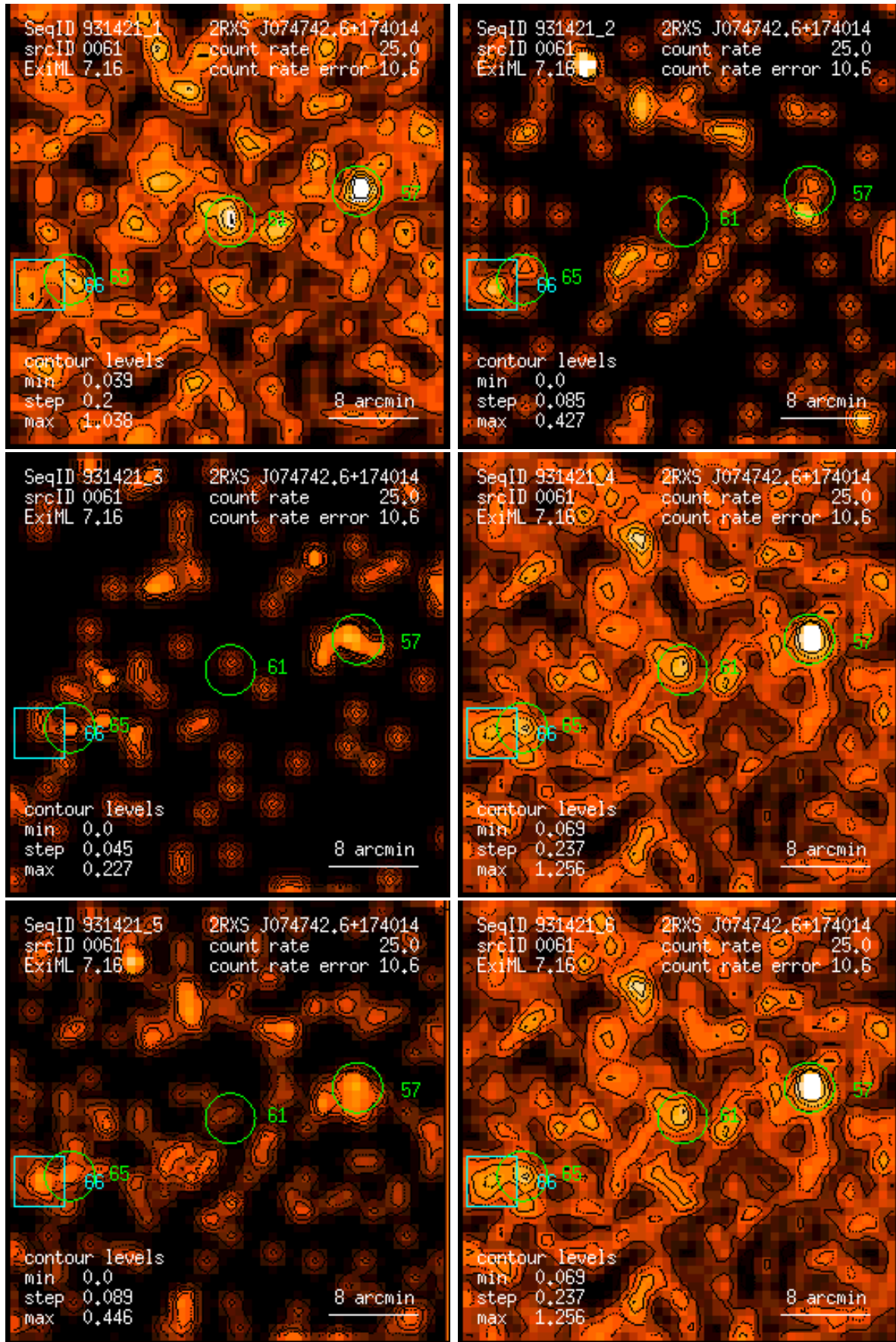
Figure 61: RASS 931421: detection 0061: band rate images, Gaussian filter: (1) PSPC channels 11 – 41, (2) 52 – 90, (3) 91 – 201, (4) 11 – 235, (5) 52 – 201, (6) 11 – 201. Broad band rates in counts/ks. Band rate contour levels in counts/ks/arcmin 2 .
