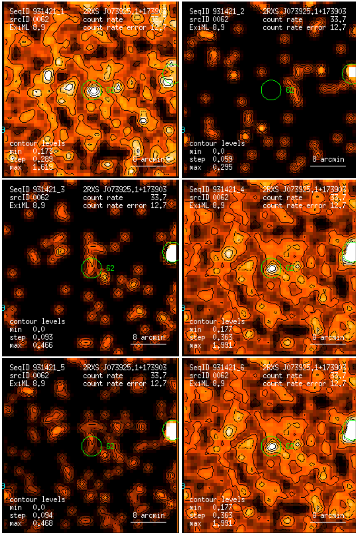
Figure 62: RASS 931421: detection 0062: band rate images, Gaussian filter: (1) PSPC channels 11 – 41, (2) 52 – 90, (3) 91 – 201, (4) 11 – 235, (5) 52 – 201, (6) 11 – 201. Broad band rates in counts/ks. Band rate contour levels in counts/ks/arcmin 2 .
