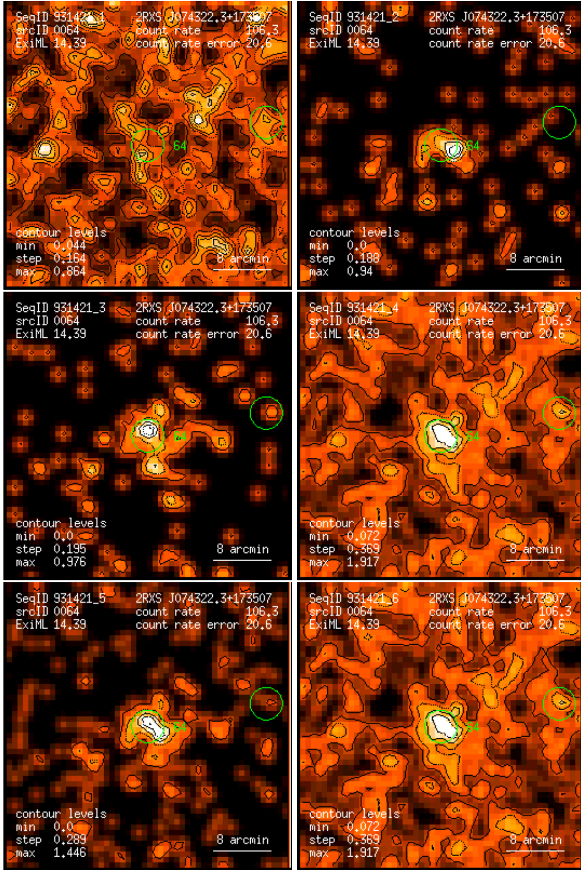
Figure 64: RASS 931421: detection 0064: band rate images, Gaussian filter: (1) PSPC channels 11 – 41, (2) 52 – 90, (3) 91 – 201, (4) 11 – 235, (5) 52 – 201, (6) 11 – 201. Broad band rates in counts/ks. Band rate contour levels in counts/ks/arcmin 2 .
