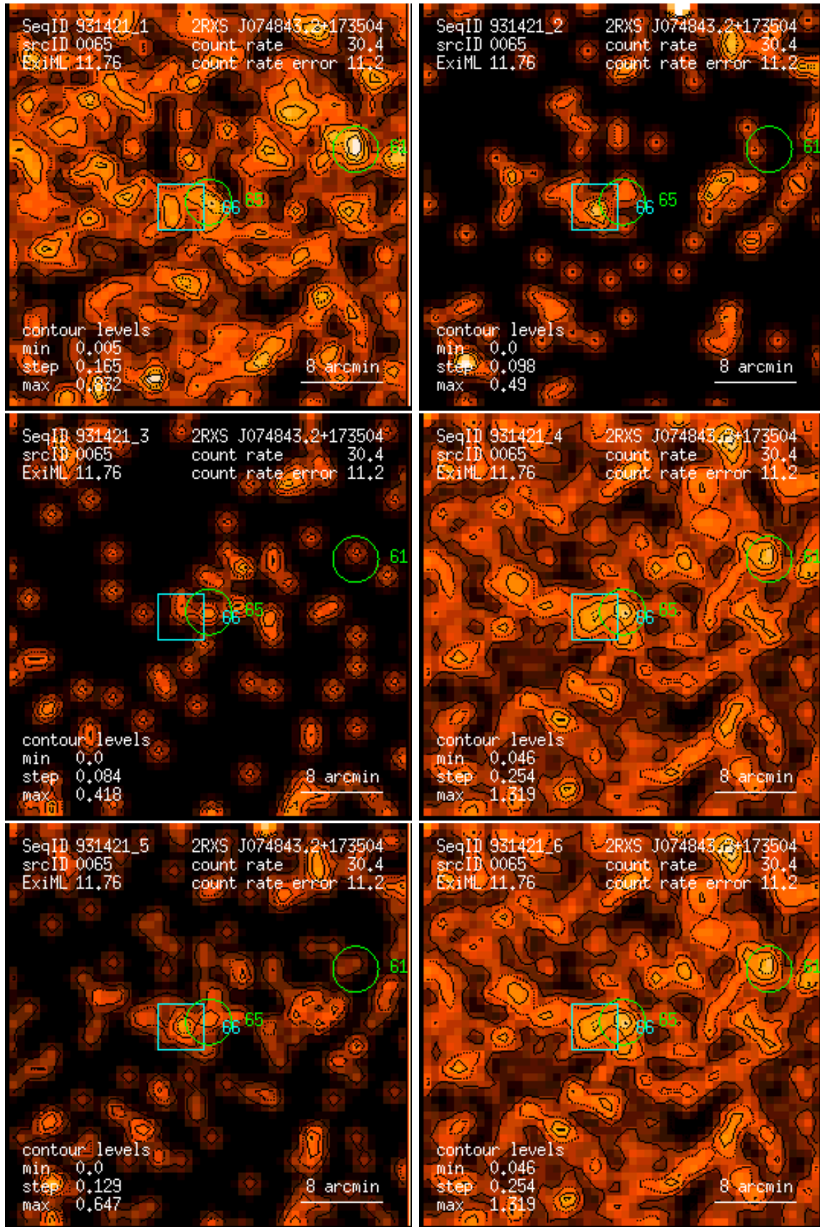
Figure 65: RASS 931421: detection 0065: band rate images, Gaussian filter: (1) PSPC channels 11 – 41, (2) 52 – 90, (3) 91 – 201, (4) 11 – 235, (5) 52 – 201, (6) 11 – 201. Broad band rates in counts/ks. Band rate contour levels in counts/ks/arcmin 2 .
