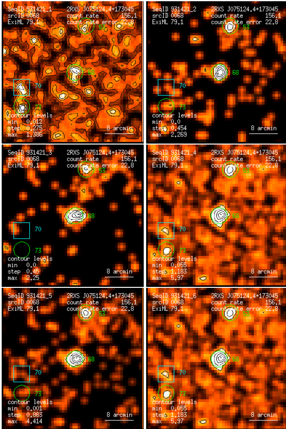
Figure 68: RASS 931421: detection 0068: band rate images, Gaussian filter: (1) PSPC channels 11 – 41, (2) 52 – 90, (3) 91 – 201, (4) 11 – 235, (5) 52 – 201, (6) 11 – 201. Broad band rates in counts/ks. Band rate contour levels in counts/ks/arcmin 2 .
