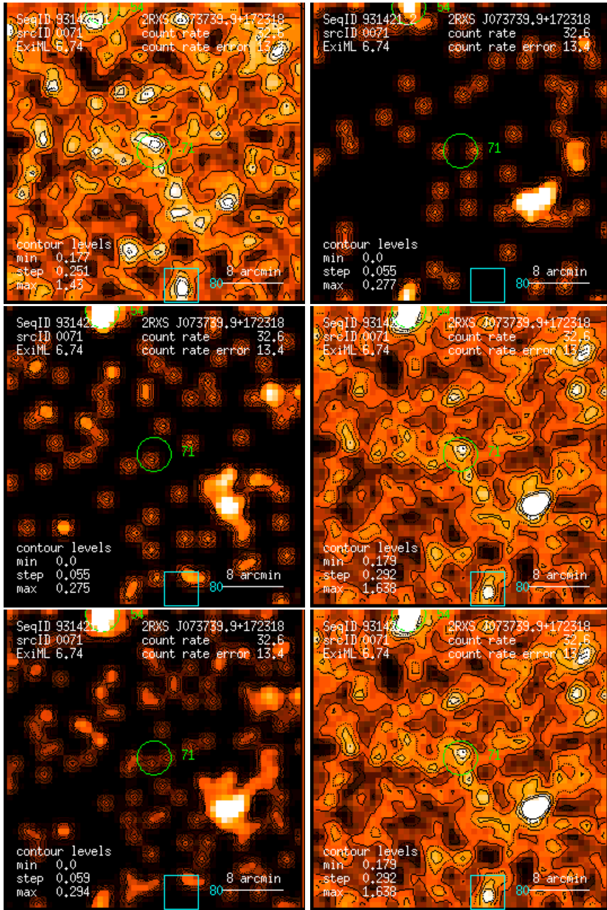
Figure 71: RASS 931421: detection 0071: band rate images, Gaussian filter: (1) PSPC channels 11 – 41, (2) 52 – 90, (3) 91 – 201, (4) 11 – 235, (5) 52 – 201, (6) 11 – 201. Broad band rates in counts/ks. Band rate contour levels in counts/ks/arcmin 2 .
