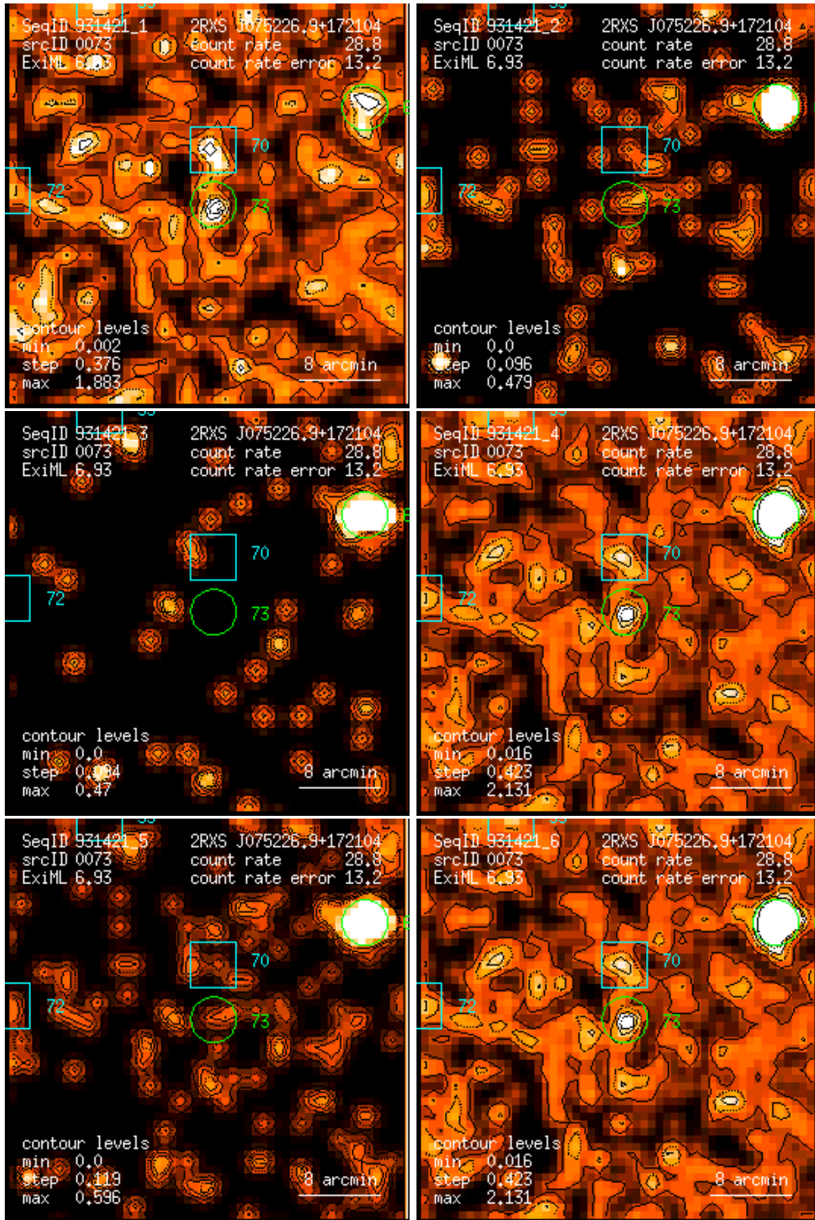
Figure 73: RASS 931421: detection 0073: band rate images, Gaussian filter: (1) PSPC channels 11 – 41, (2) 52 – 90, (3) 91 – 201, (4) 11 – 235, (5) 52 – 201, (6) 11 – 201. Broad band rates in counts/ks. Band rate contour levels in counts/ks/arcmin 2 .
