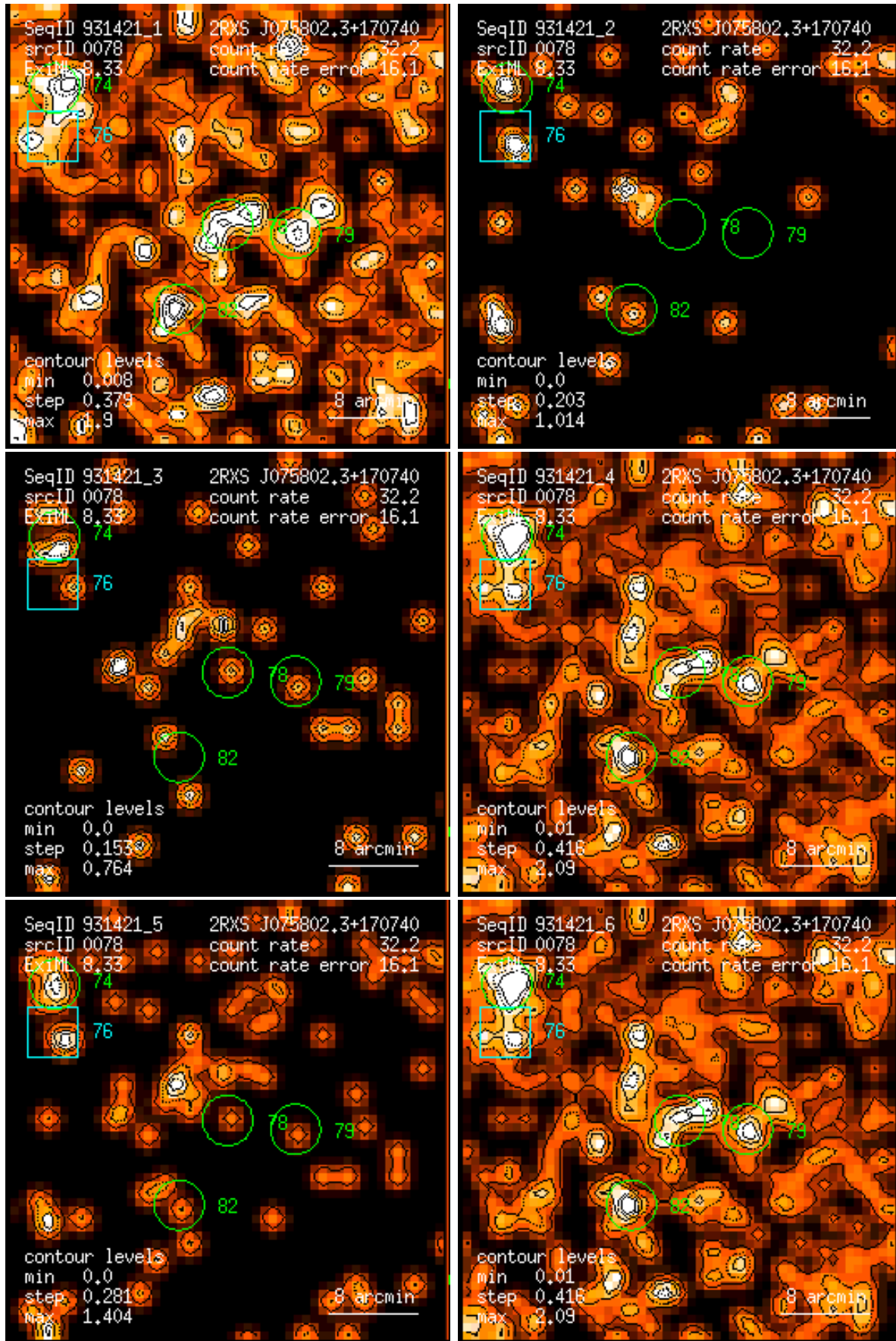
Figure 78: RASS 931421: detection 0078: band rate images, Gaussian filter: (1) PSPC channels 11 – 41, (2) 52 – 90, (3) 91 – 201, (4) 11 – 235, (5) 52 – 201, (6) 11 – 201. Broad band rates in counts/ks. Band rate contour levels in counts/ks/arcmin 2 .
