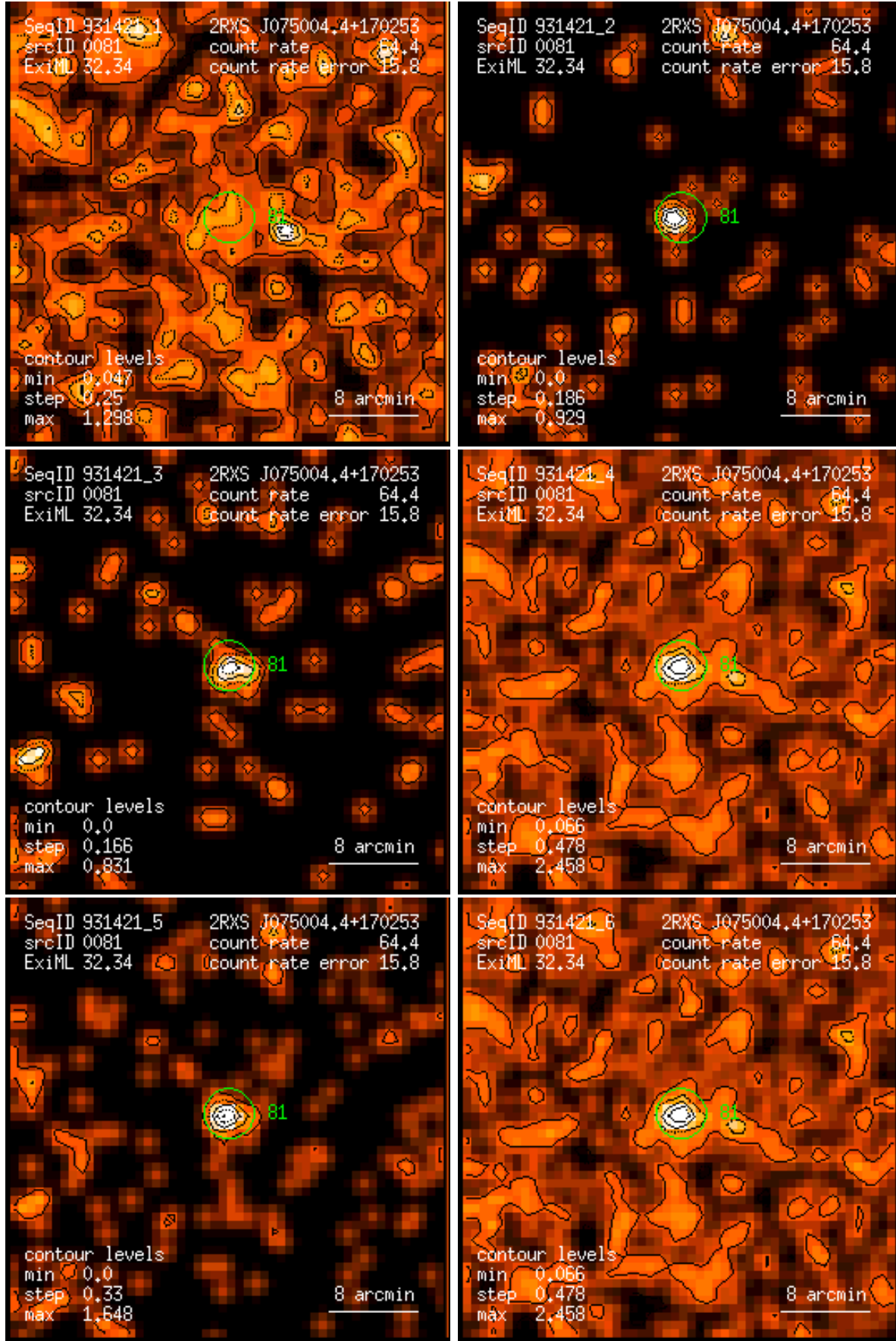
Figure 81: RASS 931421: detection 0081: band rate images, Gaussian filter: (1) PSPC channels 11 – 41, (2) 52 – 90, (3) 91 – 201, (4) 11 – 235, (5) 52 – 201, (6) 11 – 201. Broad band rates in counts/ks. Band rate contour levels in counts/ks/arcmin 2 .
