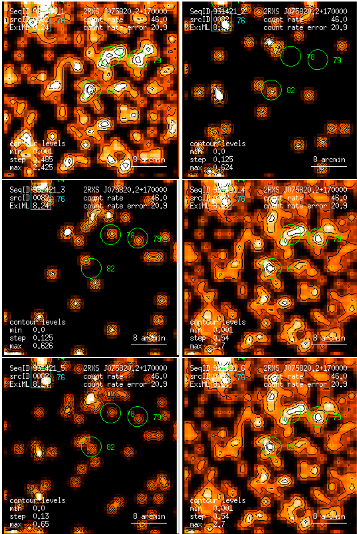
Figure 82: RASS 931421: detection 0082: band rate images, Gaussian filter: (1) PSPC channels 11 – 41, (2) 52 – 90, (3) 91 – 201, (4) 11 – 235, (5) 52 – 201, (6) 11 – 201. Broad band rates in counts/ks. Band rate contour levels in counts/ks/arcmin 2 .
