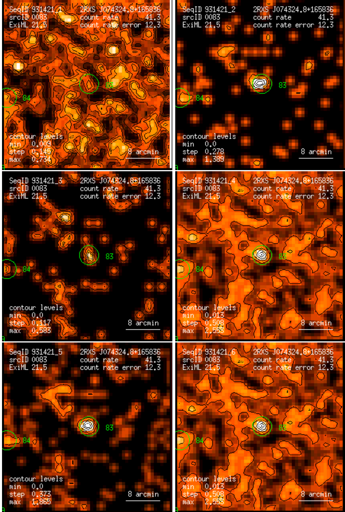
Figure 83: RASS 931421: detection 0083: band rate images, Gaussian filter: (1) PSPC channels 11 – 41, (2) 52 – 90, (3) 91 – 201, (4) 11 – 235, (5) 52 – 201, (6) 11 – 201. Broad band rates in counts/ks. Band rate contour levels in counts/ks/arcmin 2 .
