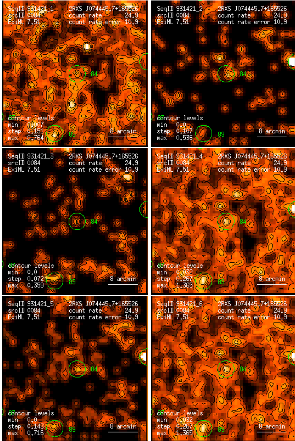
Figure 84: RASS 931421: detection 0084: band rate images, Gaussian filter: (1) PSPC channels 11 – 41, (2) 52 – 90, (3) 91 – 201, (4) 11 – 235, (5) 52 – 201, (6) 11 – 201. Broad band rates in counts/ks. Band rate contour levels in counts/ks/arcmin 2 .
