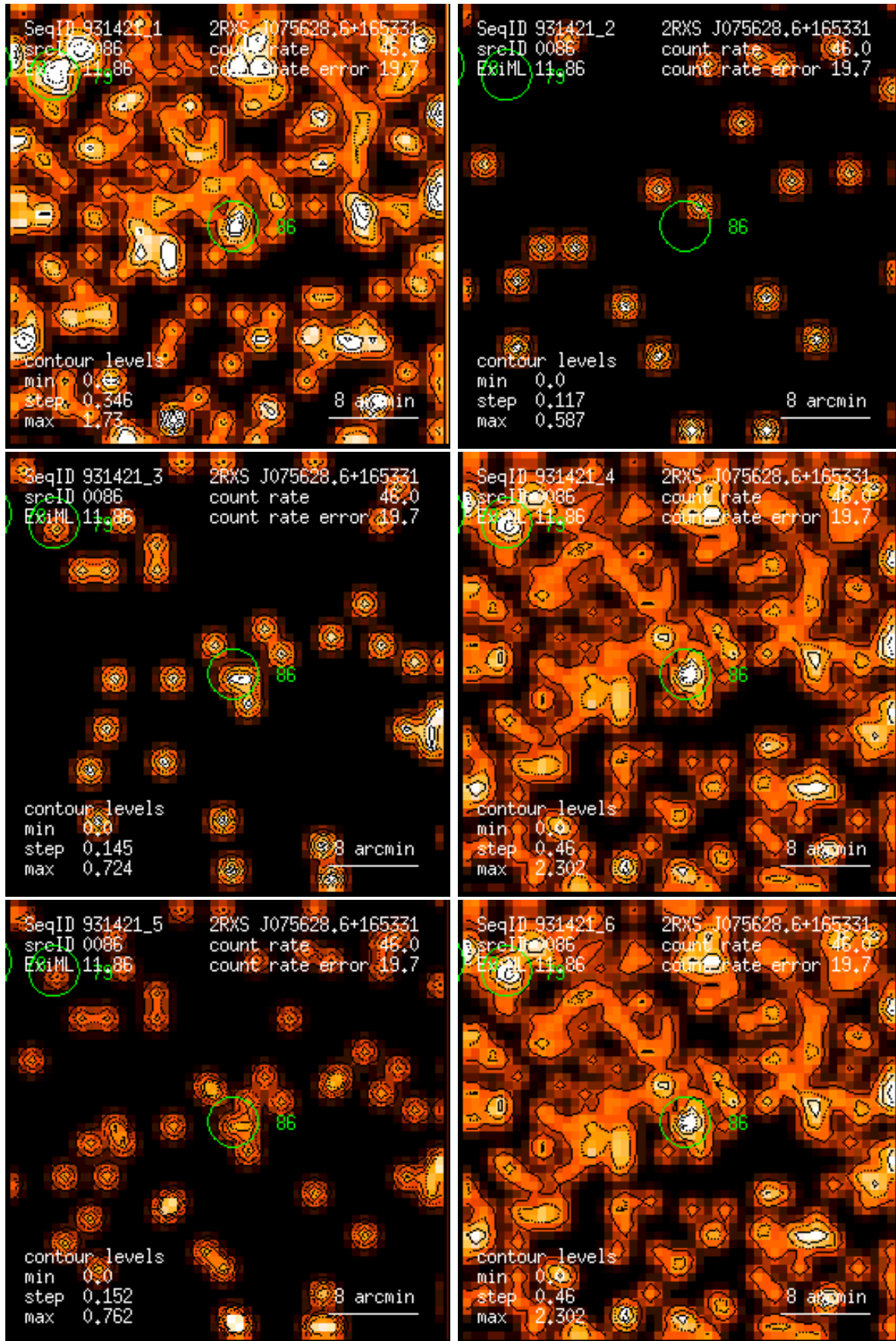
Figure 86: RASS 931421: detection 0086: band rate images, Gaussian filter: (1) PSPC channels 11 – 41, (2) 52 – 90, (3) 91 – 201, (4) 11 – 235, (5) 52 – 201, (6) 11 – 201. Broad band rates in counts/ks. Band rate contour levels in counts/ks/arcmin 2 .
