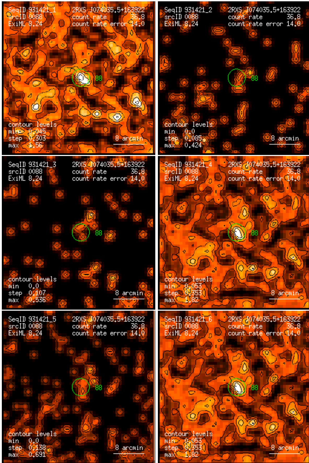
Figure 88: RASS 931421: detection 0088: band rate images, Gaussian filter: (1) PSPC channels 11 – 41, (2) 52 – 90, (3) 91 – 201, (4) 11 – 235, (5) 52 – 201, (6) 11 – 201. Broad band rates in counts/ks. Band rate contour levels in counts/ks/arcmin 2 .
