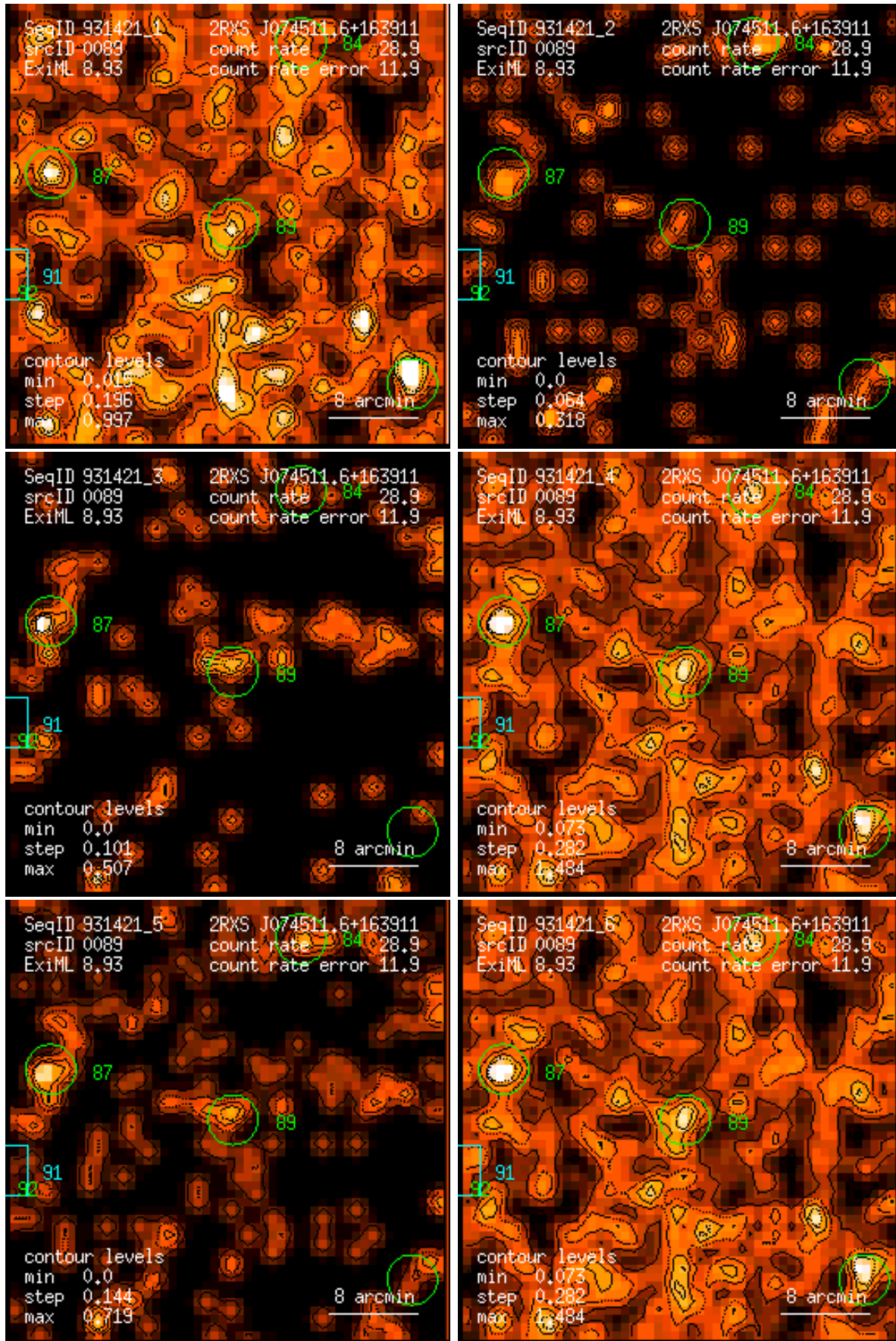
Figure 89: RASS 931421: detection 0089: band rate images, Gaussian filter: (1) PSPC channels 11 – 41, (2) 52 – 90, (3) 91 – 201, (4) 11 – 235, (5) 52 – 201, (6) 11 – 201. Broad band rates in counts/ks. Band rate contour levels in counts/ks/arcmin 2 .
