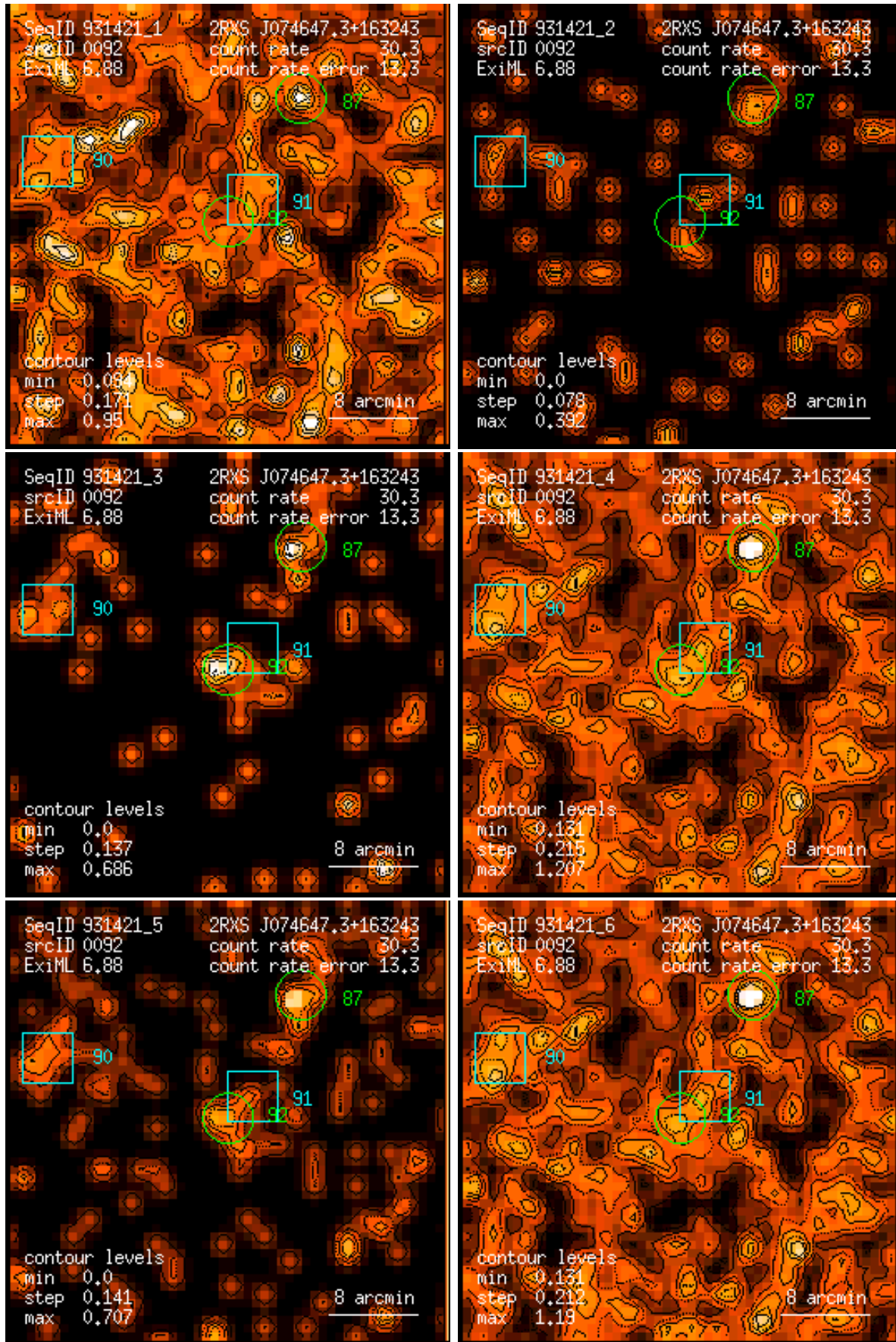
Figure 92: RASS 931421: detection 0092: band rate images, Gaussian filter: (1) PSPC channels 11 – 41, (2) 52 – 90, (3) 91 – 201, (4) 11 – 235, (5) 52 – 201, (6) 11 – 201. Broad band rates in counts/ks. Band rate contour levels in counts/ks/arcmin 2 .
