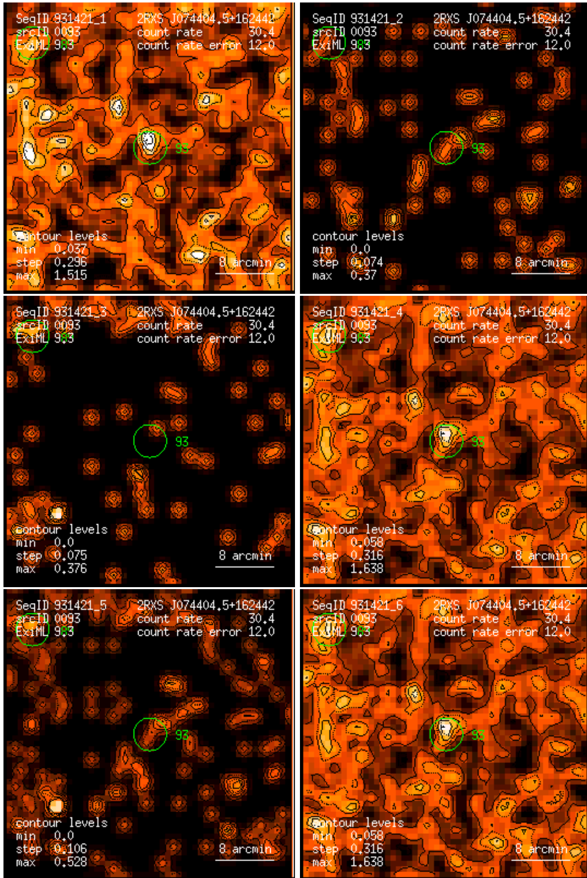
Figure 93: RASS 931421: detection 0093: band rate images, Gaussian filter: (1) PSPC channels 11 – 41, (2) 52 – 90, (3) 91 – 201, (4) 11 – 235, (5) 52 – 201, (6) 11 – 201. Broad band rates in counts/ks. Band rate contour levels in counts/ks/arcmin 2 .
