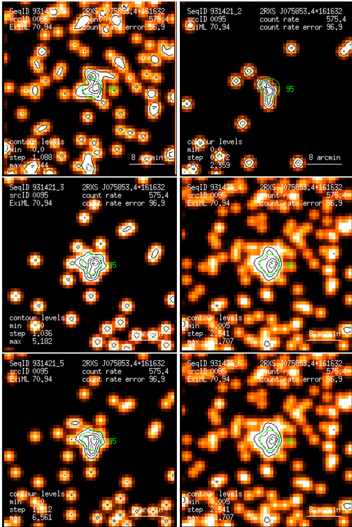
Figure 95: RASS 931421: detection 0095: band rate images, Gaussian filter: (1) PSPC channels 11 – 41, (2) 52 – 90, (3) 91 – 201, (4) 11 – 235, (5) 52 – 201, (6) 11 – 201. Broad band rates in counts/ks. Band rate contour levels in counts/ks/arcmin 2 .
