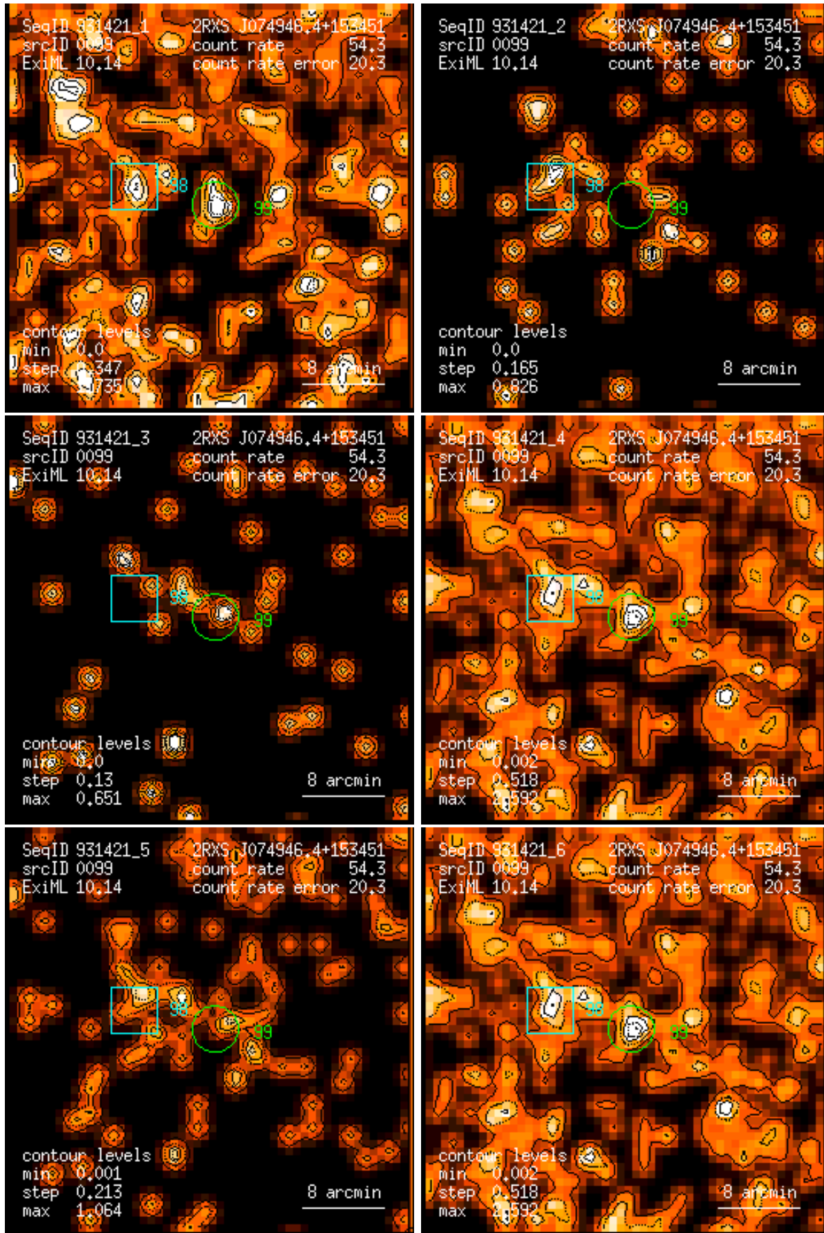
Figure 99: RASS 931421: detection 0099: band rate images, Gaussian filter: (1) PSPC channels 11 – 41, (2) 52 – 90, (3) 91 – 201, (4) 11 – 235, (5) 52 – 201, (6) 11 – 201. Broad band rates in counts/ks. Band rate contour levels in counts/ks/arcmin 2 .
