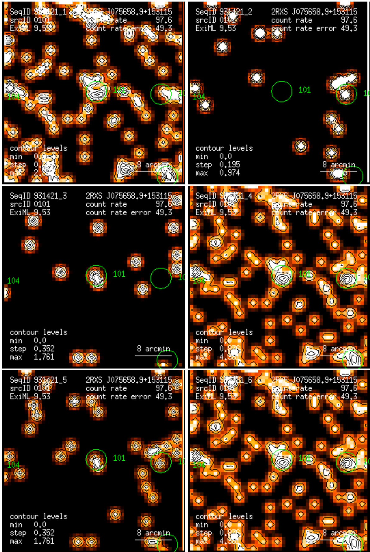
Figure 101: RASS 931421: detection 0101: band rate images, Gaussian filter: (1) PSPC channels 11 – 41, (2) 52 – 90, (3) 91 – 201, (4) 11 – 235, (5) 52 – 201, (6) 11 – 201. Broad band rates in counts/ks. Band rate contour levels in counts/ks/arcmin 2 .
