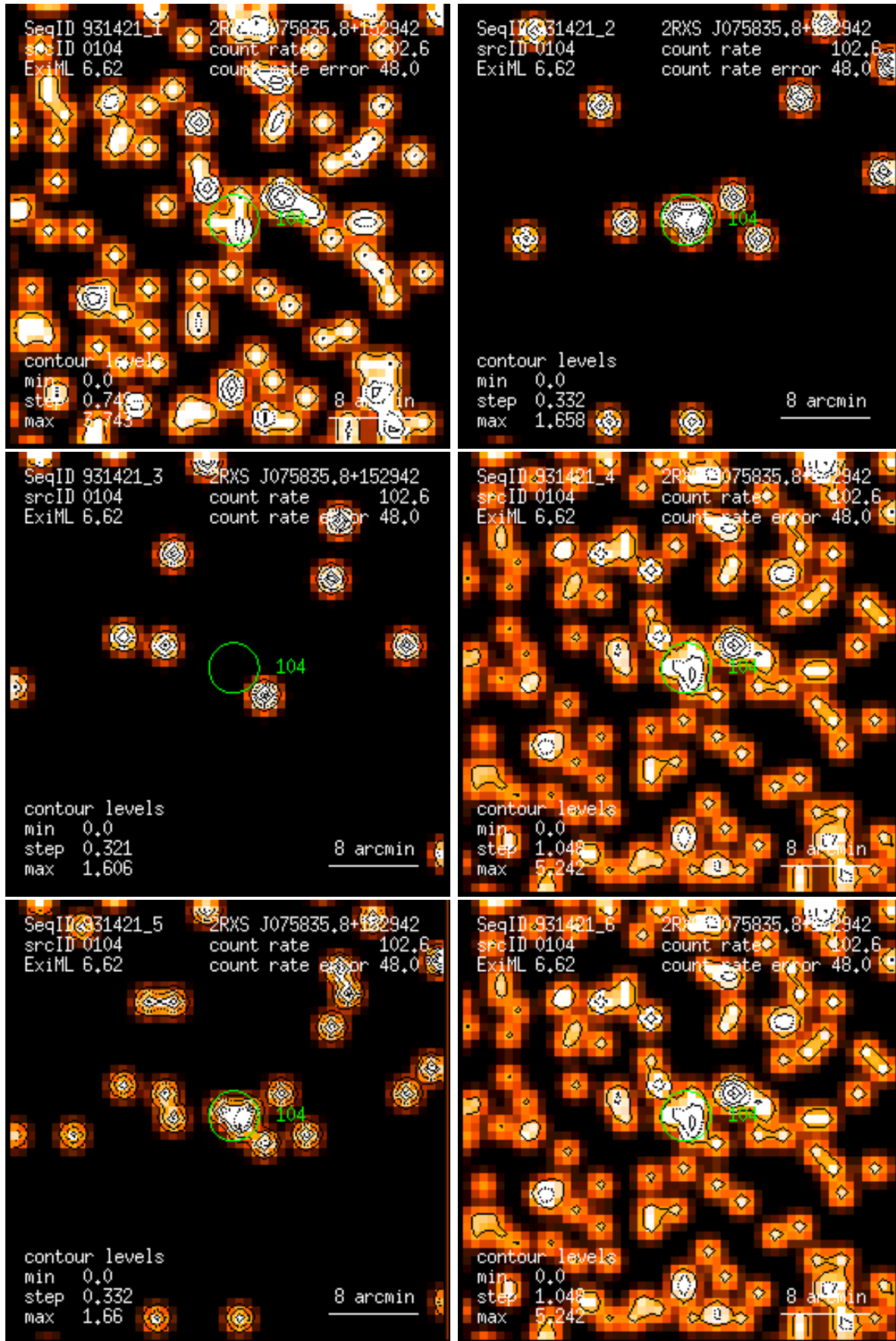
Figure 104: RASS 931421: detection 0104: band rate images, Gaussian filter: (1) PSPC channels 11 – 41, (2) 52 – 90, (3) 91 – 201, (4) 11 – 235, (5) 52 – 201, (6) 11 – 201. Broad band rates in counts/ks. Band rate contour levels in counts/ks/arcmin 2 .
