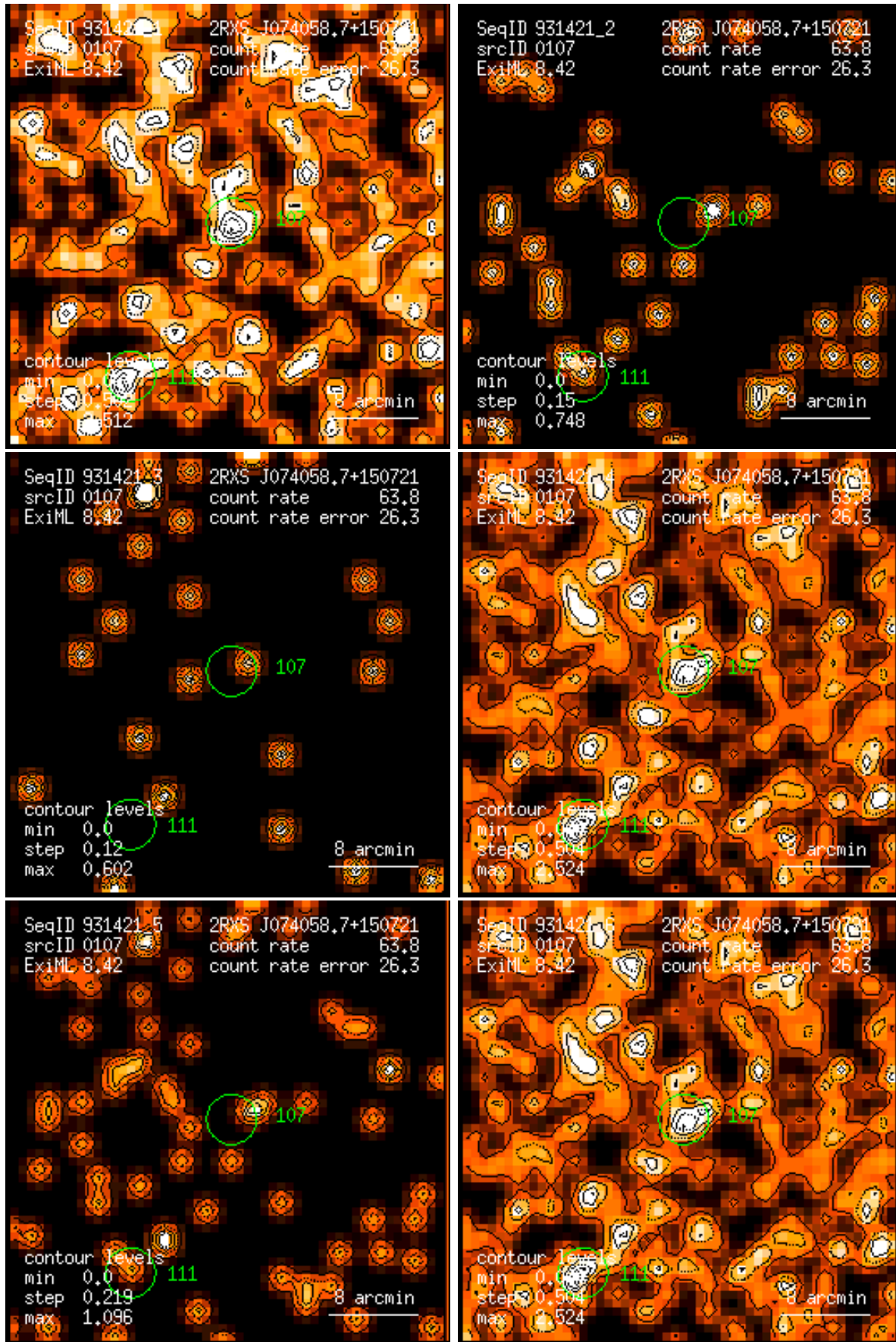
Figure 107: RASS 931421: detection 0107: band rate images, Gaussian filter: (1) PSPC channels 11 – 41, (2) 52 – 90, (3) 91 – 201, (4) 11 – 235, (5) 52 – 201, (6) 11 – 201. Broad band rates in counts/ks. Band rate contour levels in counts/ks/arcmin 2 .
