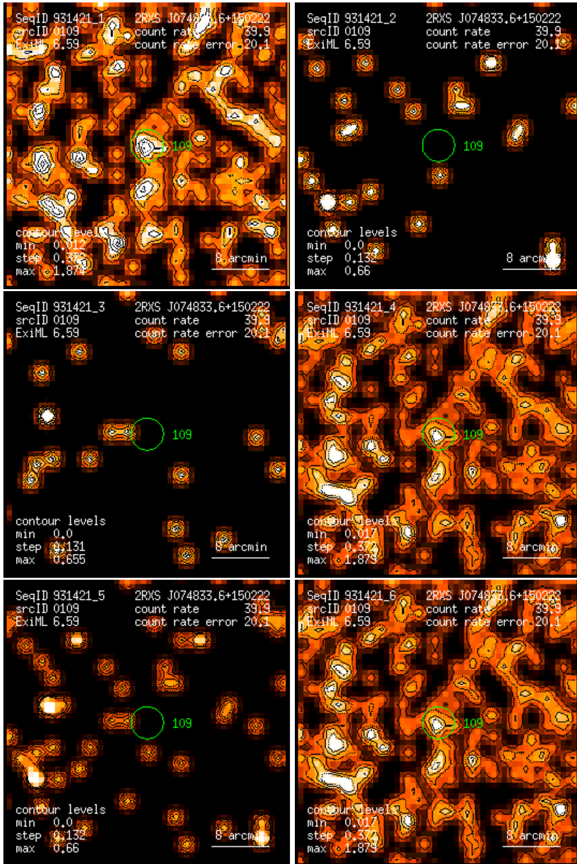
Figure 109: RASS 931421: detection 0109: band rate images, Gaussian filter: (1) PSPC channels 11 – 41, (2) 52 – 90, (3) 91 – 201, (4) 11 – 235, (5) 52 – 201, (6) 11 – 201. Broad band rates in counts/ks. Band rate contour levels in counts/ks/arcmin 2 .
