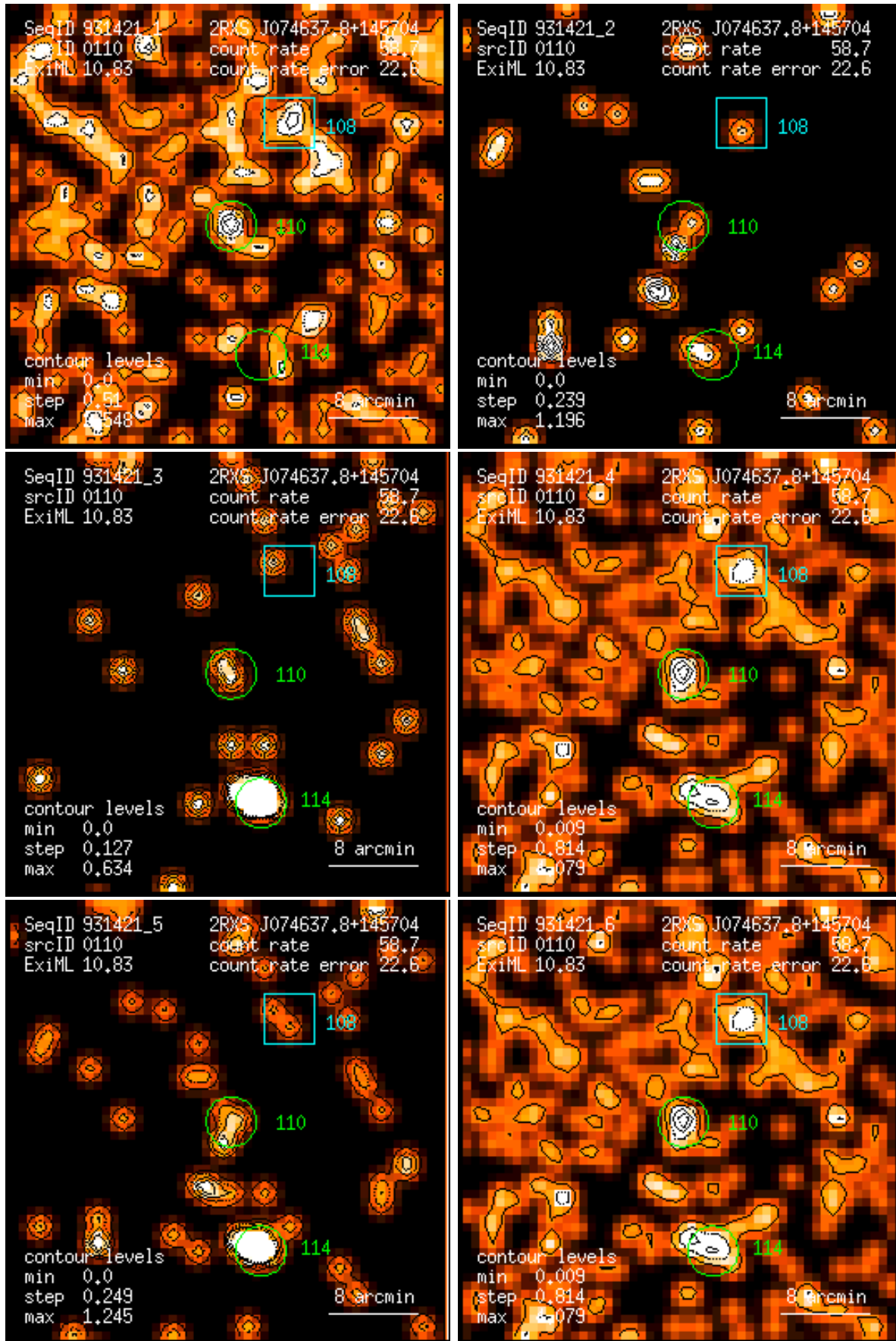
Figure 110: RASS 931421: detection 0110: band rate images, Gaussian filter: (1) PSPC channels 11 – 41, (2) 52 – 90, (3) 91 – 201, (4) 11 – 235, (5) 52 – 201, (6) 11 – 201. Broad band rates in counts/ks. Band rate contour levels in counts/ks/arcmin 2 .
