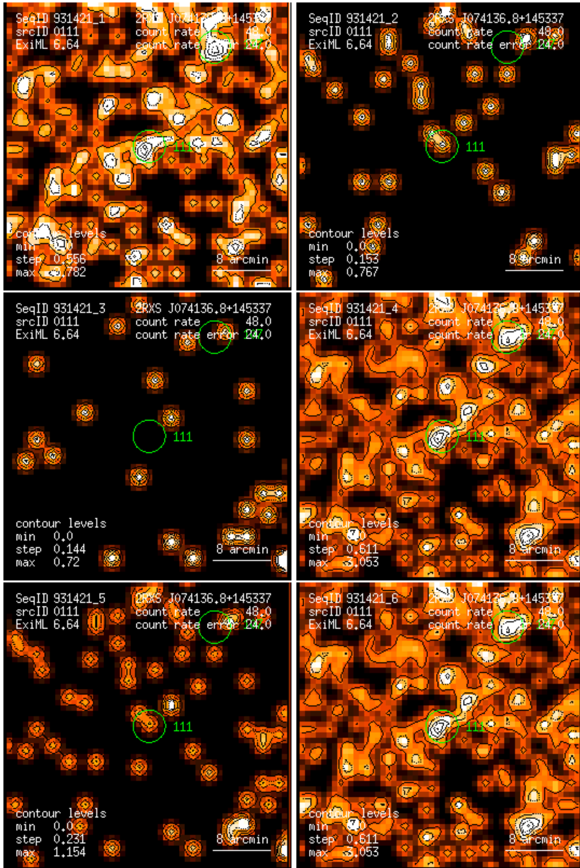
Figure 111: RASS 931421: detection 0111: band rate images, Gaussian filter: (1) PSPC channels 11 – 41, (2) 52 – 90, (3) 91 – 201, (4) 11 – 235, (5) 52 – 201, (6) 11 – 201. Broad band rates in counts/ks. Band rate contour levels in counts/ks/arcmin 2 .
