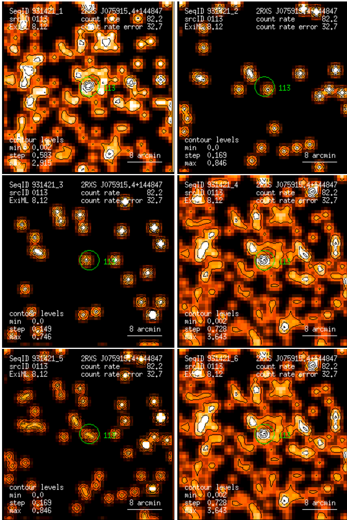
Figure 113: RASS 931421: detection 0113: band rate images, Gaussian filter: (1) PSPC channels 11 – 41, (2) 52 – 90, (3) 91 – 201, (4) 11 – 235, (5) 52 – 201, (6) 11 – 201. Broad band rates in counts/ks. Band rate contour levels in counts/ks/arcmin 2 .
