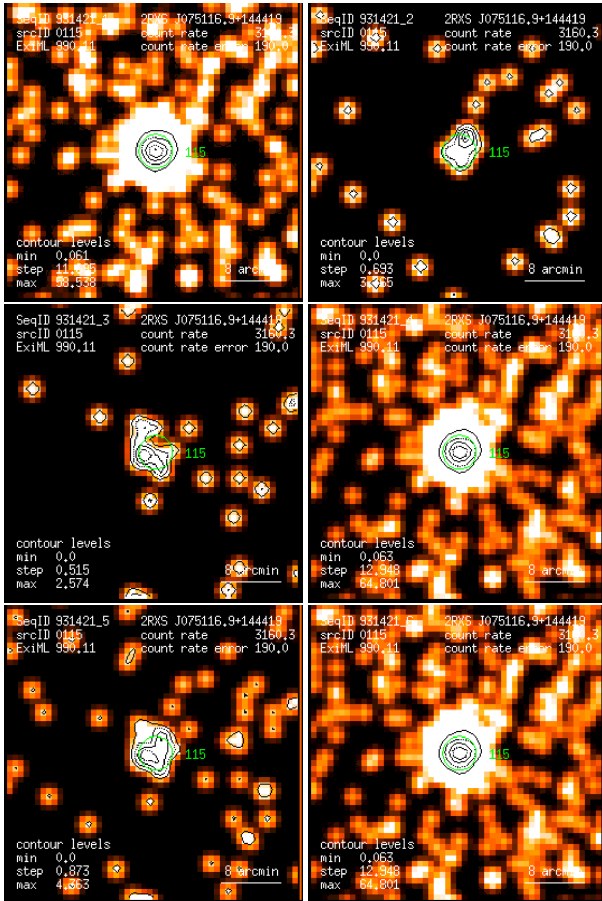
Figure 115: RASS 931421: detection 0115: band rate images, Gaussian filter: (1) PSPC channels 11 – 41, (2) 52 – 90, (3) 91 – 201, (4) 11 – 235, (5) 52 – 201, (6) 11 – 201. Broad band rates in counts/ks. Band rate contour levels in counts/ks/arcmin 2 .
