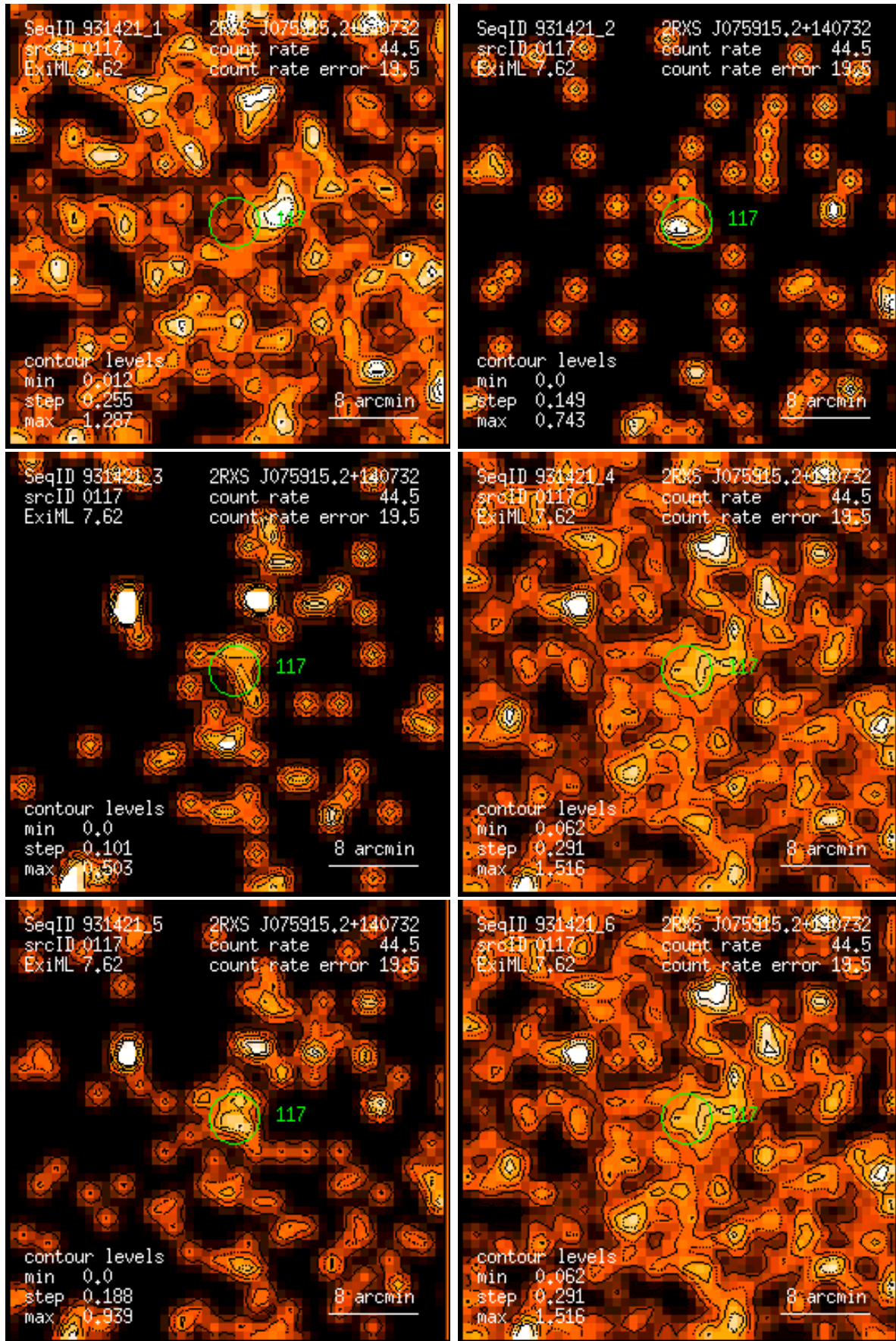
Figure 117: RASS 931421: detection 0117: band rate images, Gaussian filter: (1) PSPC channels 11 – 41, (2) 52 – 90, (3) 91 – 201, (4) 11 – 235, (5) 52 – 201, (6) 11 – 201. Broad band rates in counts/ks. Band rate contour levels in counts/ks/arcmin 2 .
