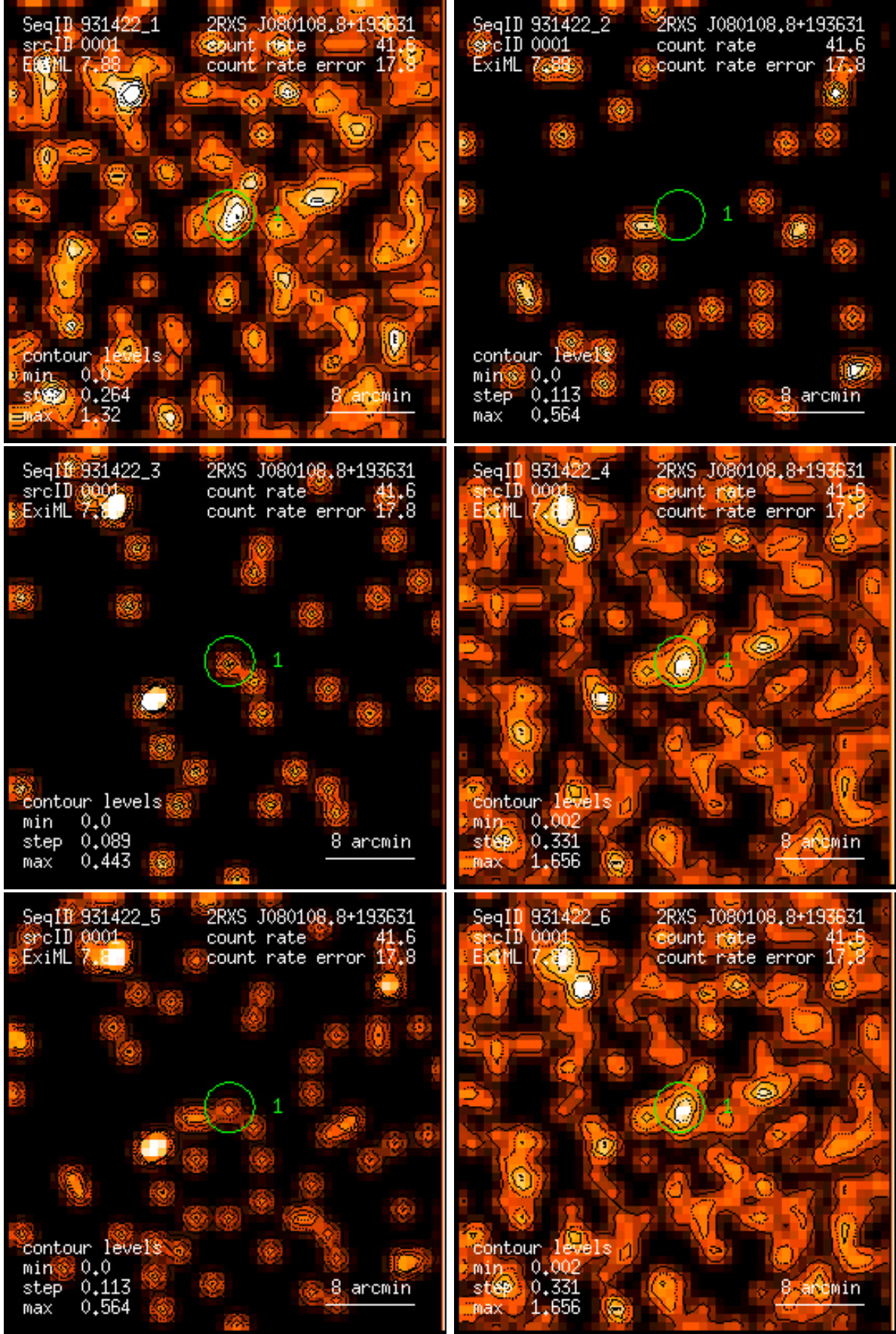
Figure 1: RASS 931422: detection 0001: band rate images, Gaussian filter: (1) PSPC channels 11 – 41, (2) 52 – 90, (3) 91 – 201, (4) 11 – 235, (5) 52 – 201, (6) 11 – 201. Broad band rates in counts/ks. Band rate contour levels in counts/ks/arcmin 2 .
