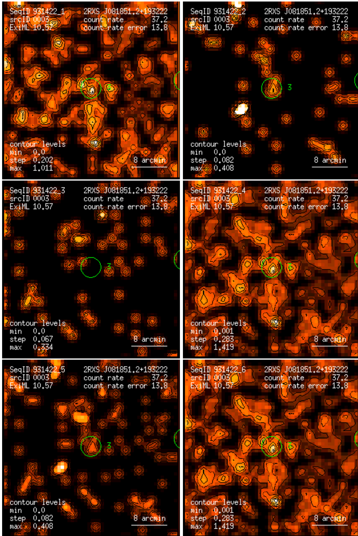
Figure 3: RASS 931422: detection 0003: band rate images, Gaussian filter: (1) PSPC channels 11 – 41, (2) 52 – 90, (3) 91 – 201, (4) 11 – 235, (5) 52 – 201, (6) 11 – 201. Broad band rates in counts/ks. Band rate contour levels in counts/ks/arcmin 2 .
