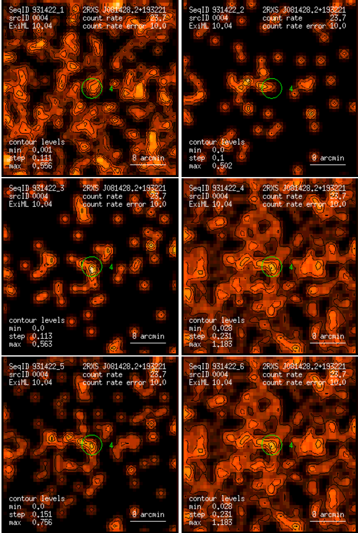
Figure 4: RASS 931422: detection 0004: band rate images, Gaussian filter: (1) PSPC channels 11 – 41, (2) 52 – 90, (3) 91 – 201, (4) 11 – 235, (5) 52 – 201, (6) 11 – 201. Broad band rates in counts/ks. Band rate contour levels in counts/ks/arcmin 2 .
