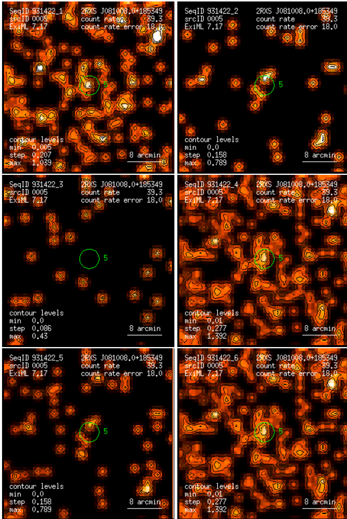
Figure 5: RASS 931422: detection 0005: band rate images, Gaussian filter: (1) PSPC channels 11 – 41, (2) 52 – 90, (3) 91 – 201, (4) 11 – 235, (5) 52 – 201, (6) 11 – 201. Broad band rates in counts/ks. Band rate contour levels in counts/ks/arcmin 2 .
