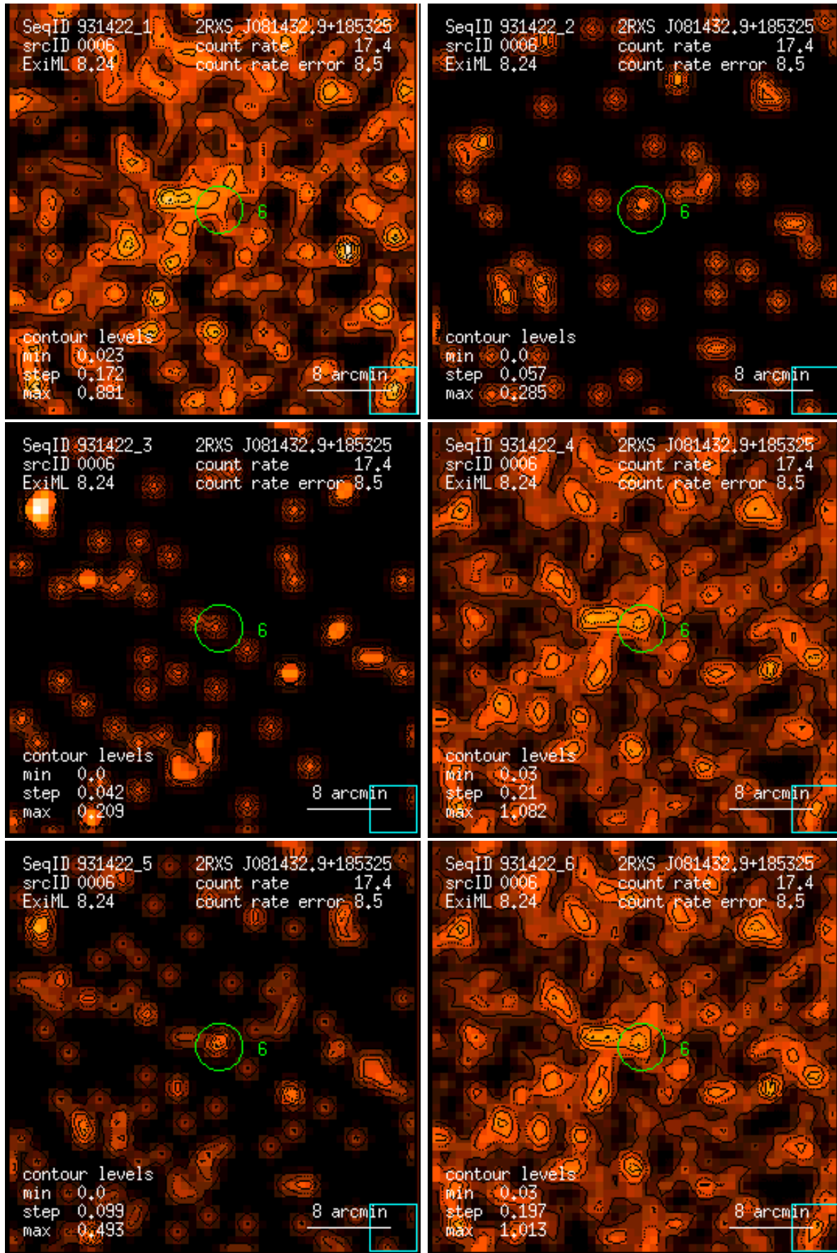
Figure 6: RASS 931422: detection 0006: band rate images, Gaussian filter: (1) PSPC channels 11 – 41, (2) 52 – 90, (3) 91 – 201, (4) 11 – 235, (5) 52 – 201, (6) 11 – 201. Broad band rates in counts/ks. Band rate contour levels in counts/ks/arcmin 2 .
