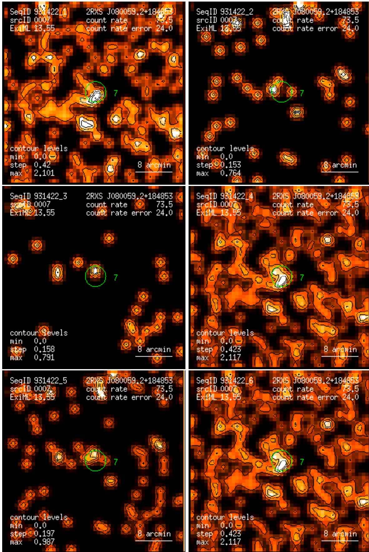
Figure 7: RASS 931422: detection 0007: band rate images, Gaussian filter: (1) PSPC channels 11 – 41, (2) 52 – 90, (3) 91 – 201, (4) 11 – 235, (5) 52 – 201, (6) 11 – 201. Broad band rates in counts/ks. Band rate contour levels in counts/ks/arcmin 2 .
