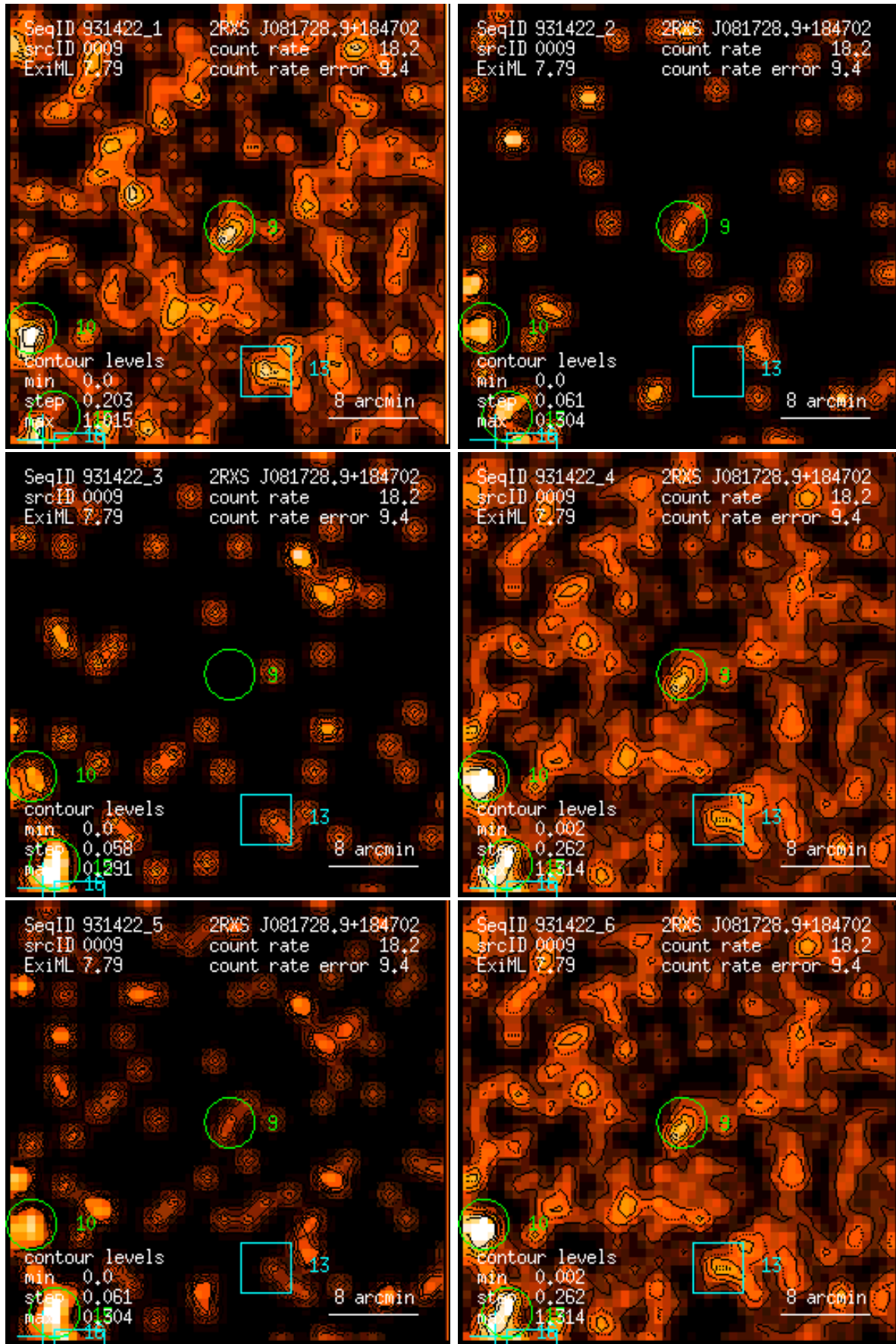
Figure 9: RASS 931422: detection 0009: band rate images, Gaussian filter: (1) PSPC channels 11 – 41, (2) 52 – 90, (3) 91 – 201, (4) 11 – 235, (5) 52 – 201, (6) 11 – 201. Broad band rates in counts/ks. Band rate contour levels in counts/ks/arcmin 2 .
