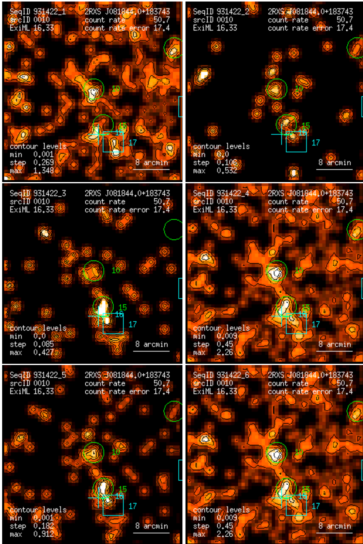
Figure 10: RASS 931422: detection 0010: band rate images, Gaussian filter: (1) PSPC channels 11 – 41, (2) 52 – 90, (3) 91 – 201, (4) 11 – 235, (5) 52 – 201, (6) 11 – 201. Broad band rates in counts/ks. Band rate contour levels in counts/ks/arcmin 2 .
