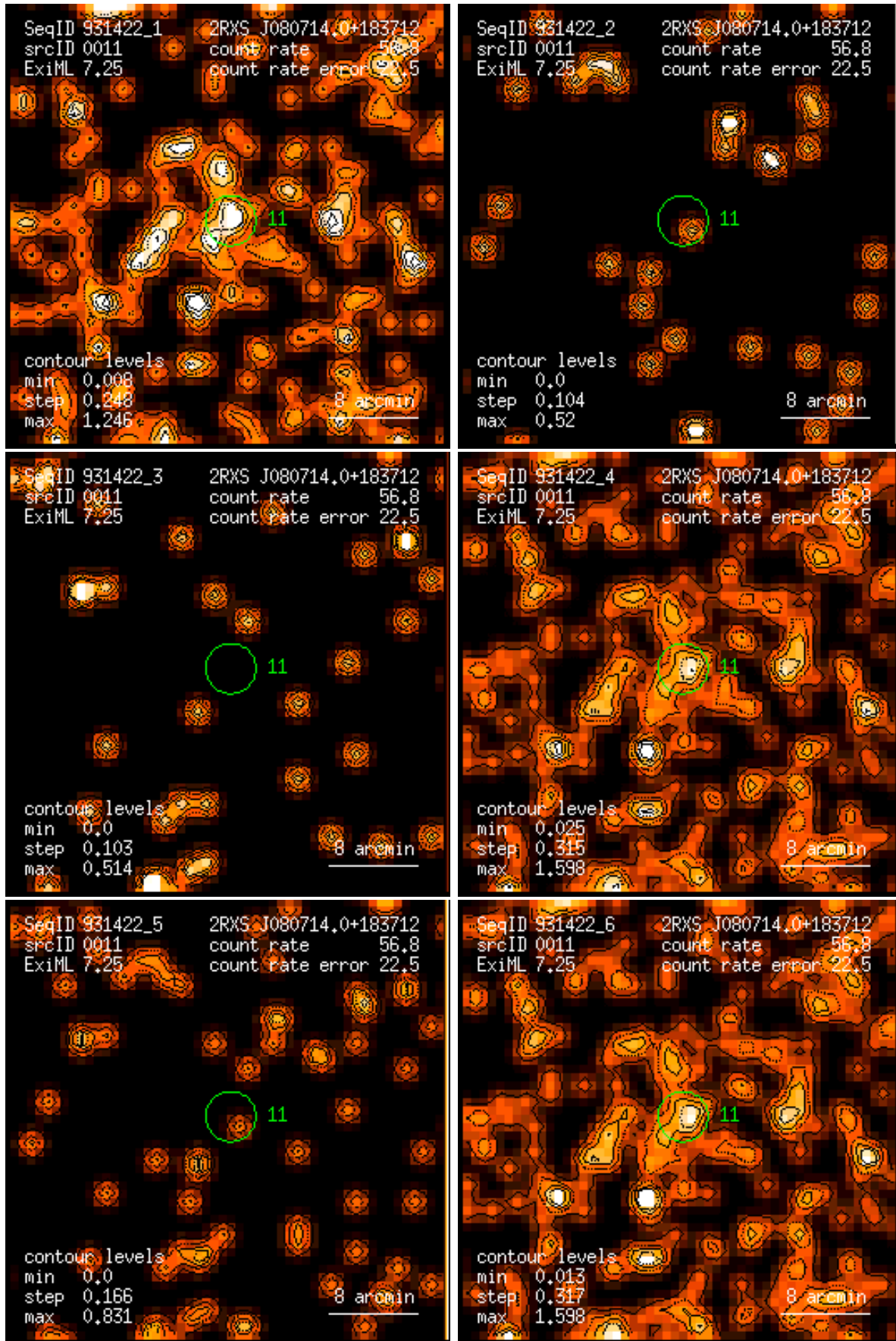
Figure 11: RASS 931422: detection 0011: band rate images, Gaussian filter: (1) PSPC channels 11 – 41, (2) 52 – 90, (3) 91 – 201, (4) 11 – 235, (5) 52 – 201, (6) 11 – 201. Broad band rates in counts/ks. Band rate contour levels in counts/ks/arcmin 2 .
