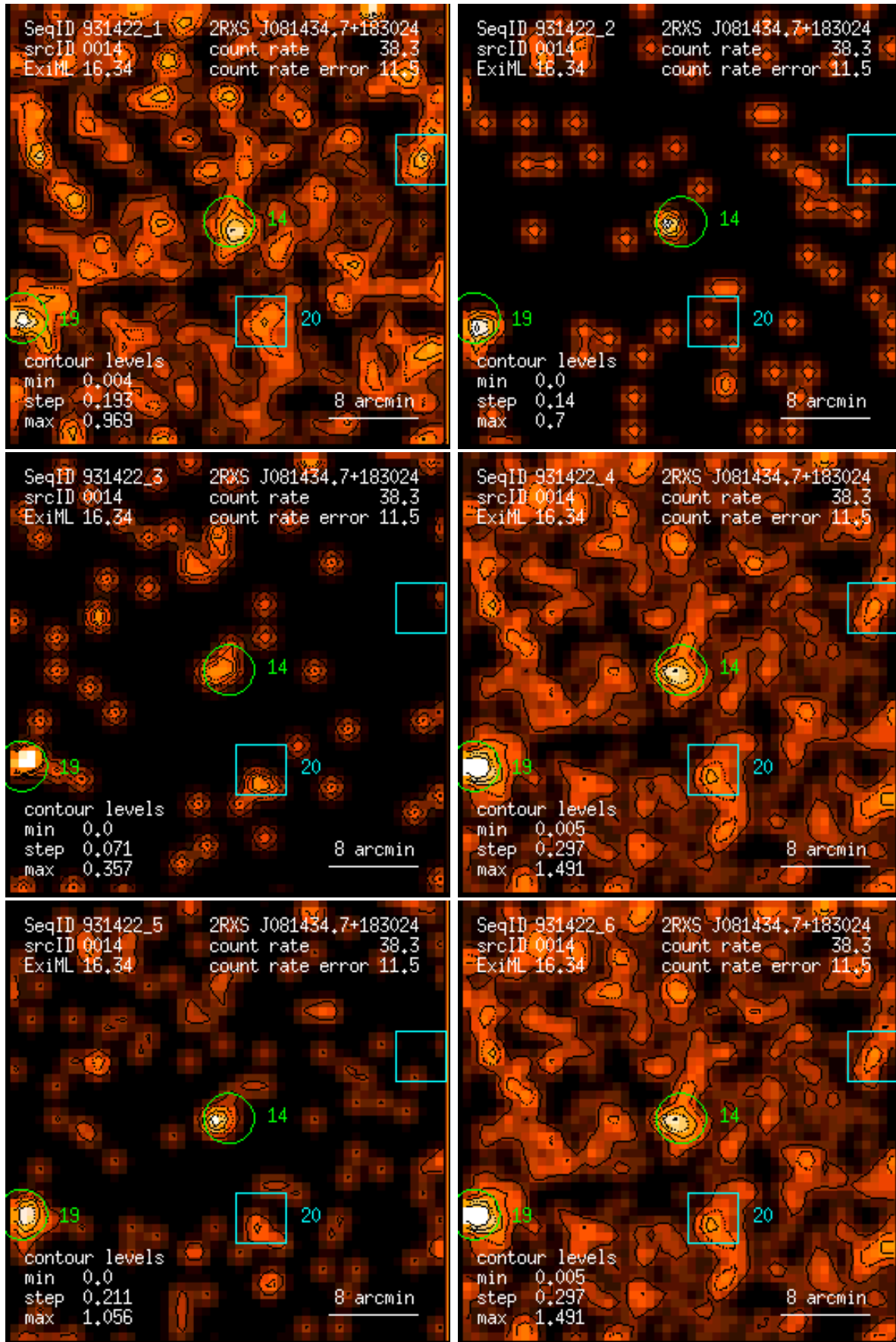
Figure 14: RASS 931422: detection 0014: band rate images, Gaussian filter: (1) PSPC channels 11 – 41, (2) 52 – 90, (3) 91 – 201, (4) 11 – 235, (5) 52 – 201, (6) 11 – 201. Broad band rates in counts/ks. Band rate contour levels in counts/ks/arcmin 2 .
