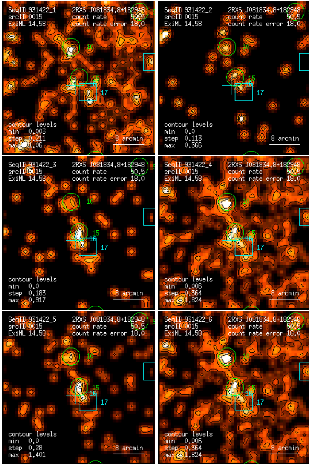
Figure 15: RASS 931422: detection 0015: band rate images, Gaussian filter: (1) PSPC channels 11 – 41, (2) 52 – 90, (3) 91 – 201, (4) 11 – 235, (5) 52 – 201, (6) 11 – 201. Broad band rates in counts/ks. Band rate contour levels in counts/ks/arcmin 2 .
