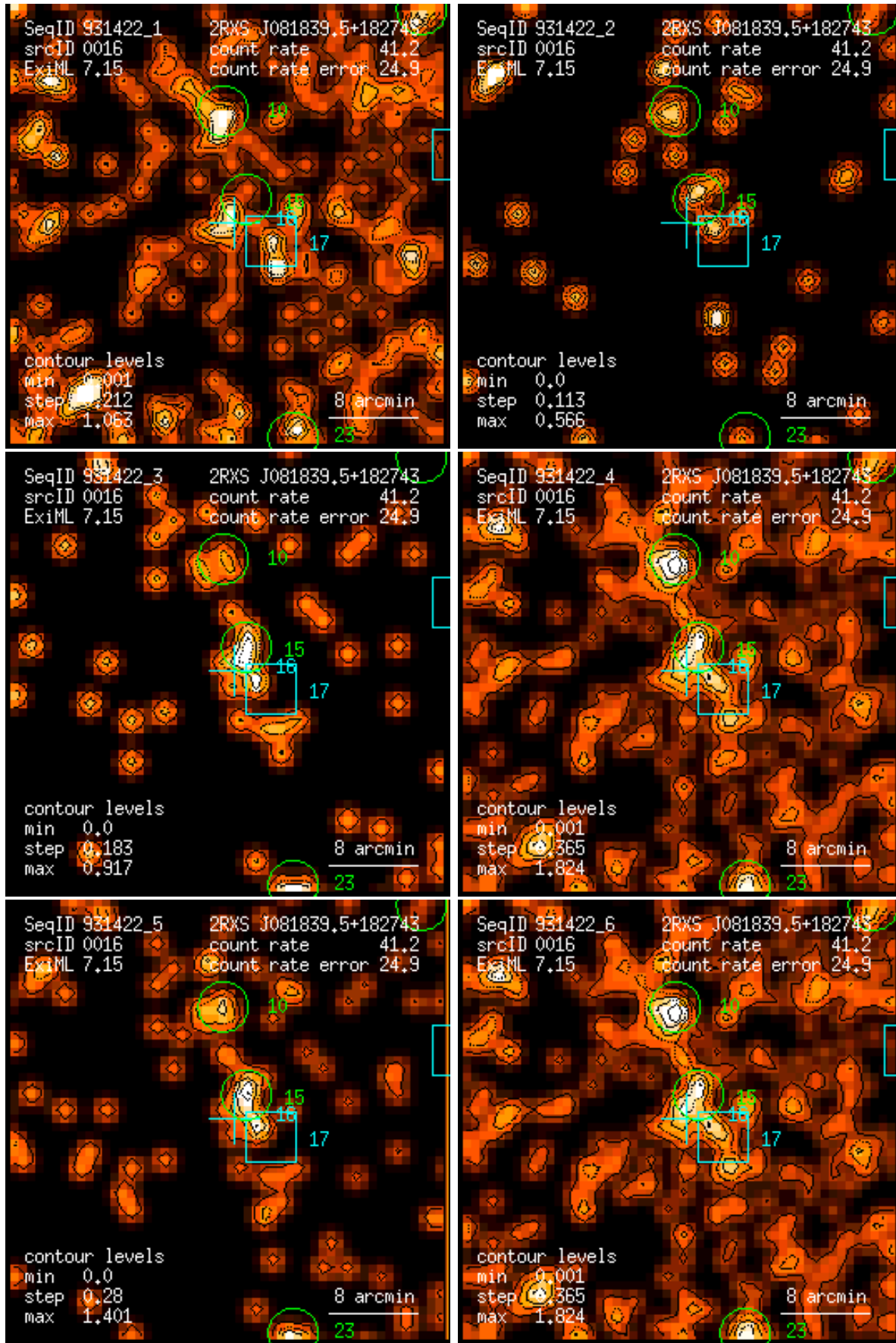
Figure 16: RASS 931422: detection 0016: band rate images, Gaussian filter: (1) PSPC channels 11 – 41, (2) 52 – 90, (3) 91 – 201, (4) 11 – 235, (5) 52 – 201, (6) 11 – 201. Broad band rates in counts/ks. Band rate contour levels in counts/ks/arcmin 2 .
